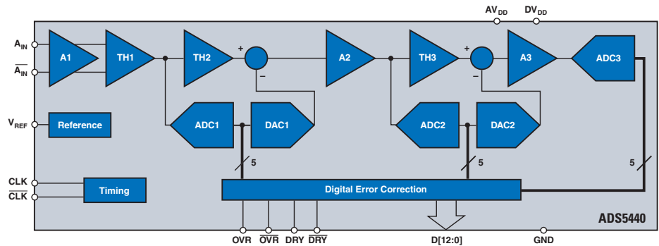
ADS5440 functional block diagram.
