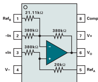
INA132 functional block diagram.
