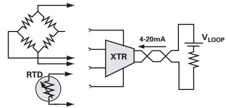
4-20mA transmitter design solutions.
