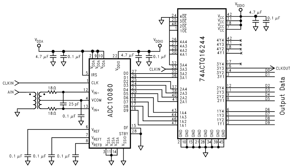
FIGURE 5. A Simple Application Using a Differentially Driving Source
