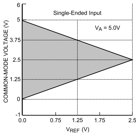
FIGURE 9. V_{CM} range for single-ended operation
