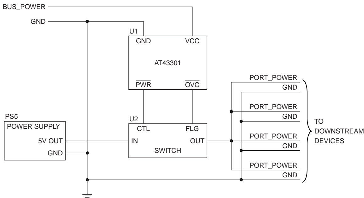
Figure 3. Self-powered Hub
