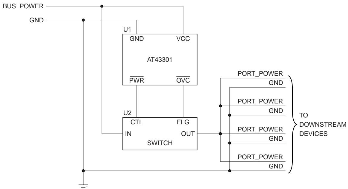
Figure 2. Bus-powered Hub
