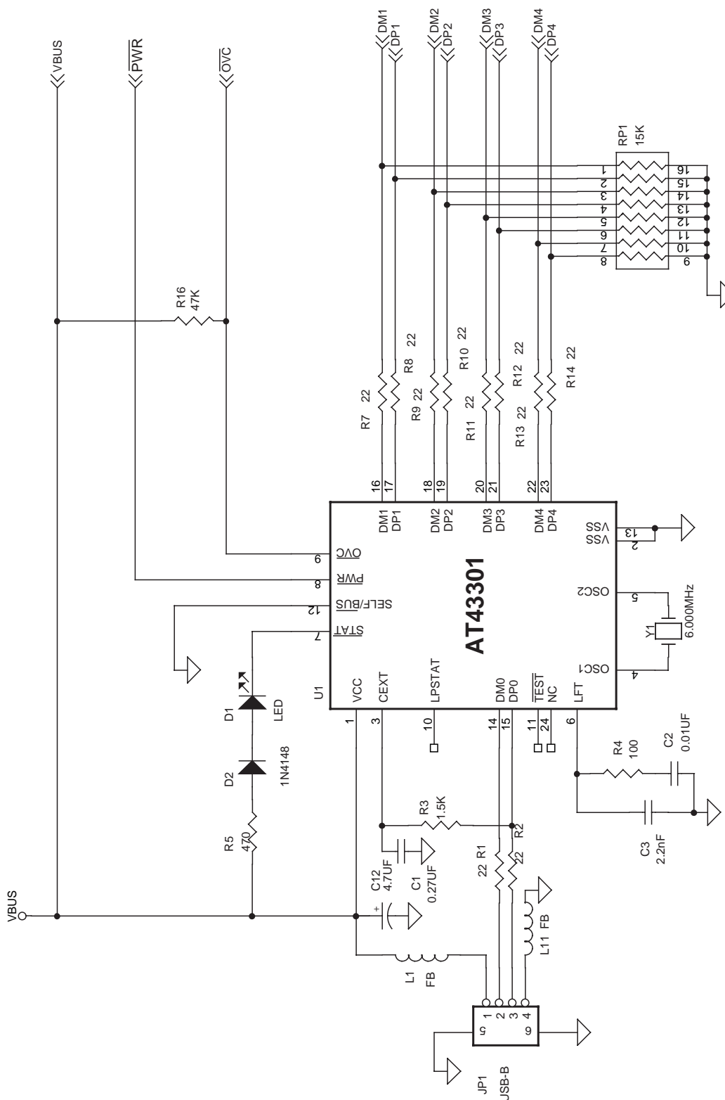
Figure 13. Bus-powered Hub
