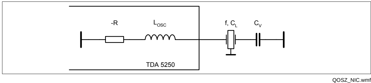
Figure 3-15 Crystal Oscillator
