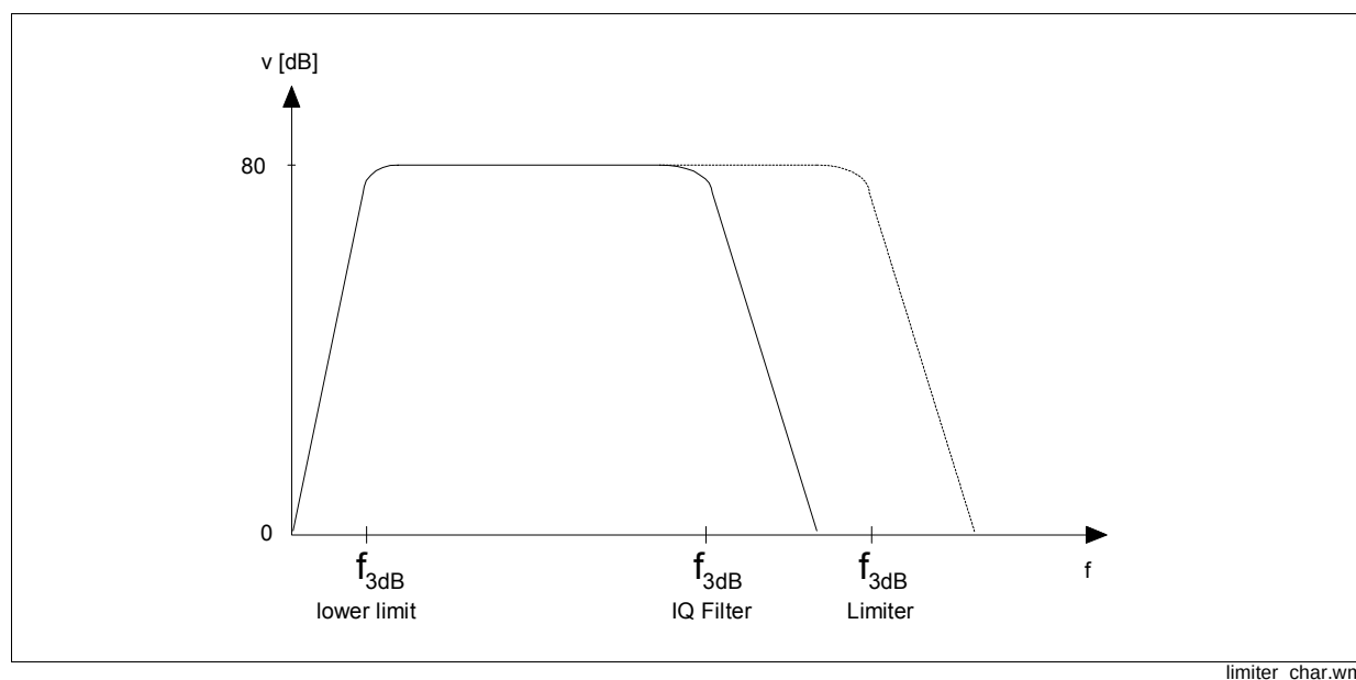
Figure 3-23 Limiter frequency characteristics
