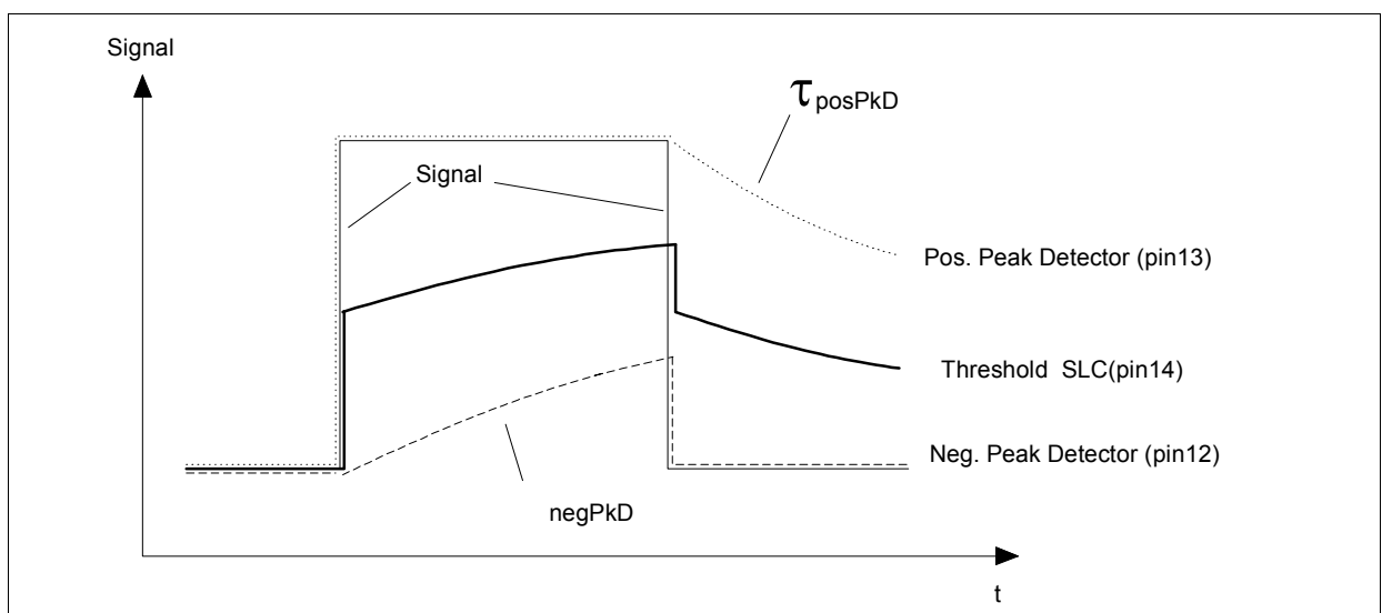
Figure 3-27 Peak Detector timing
