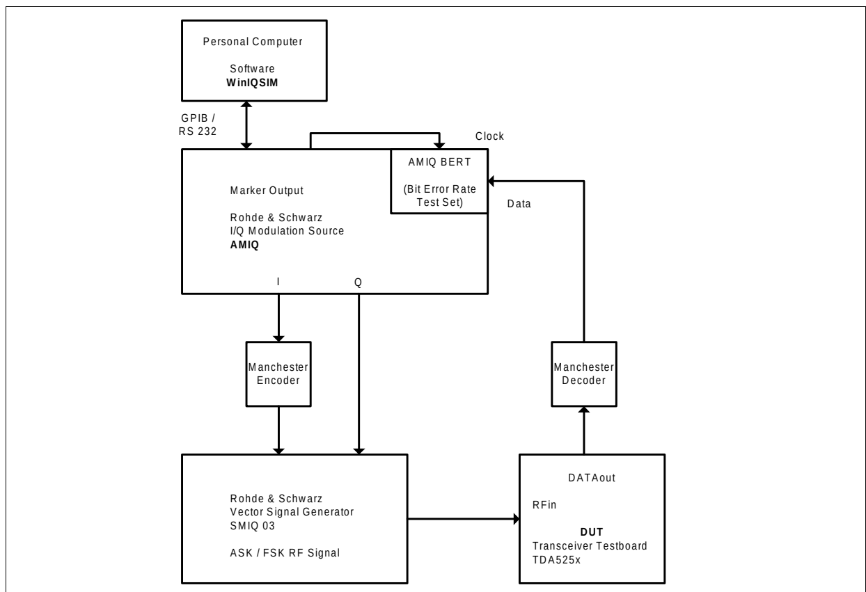
Figure 3-36 BER Test Setup
