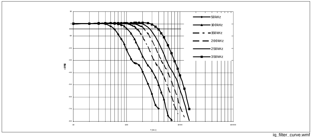
Figure 3-20 I/Q Filter Characteristics
