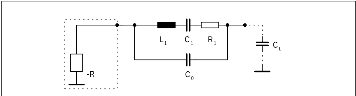
Figure 3-14 Crystal
