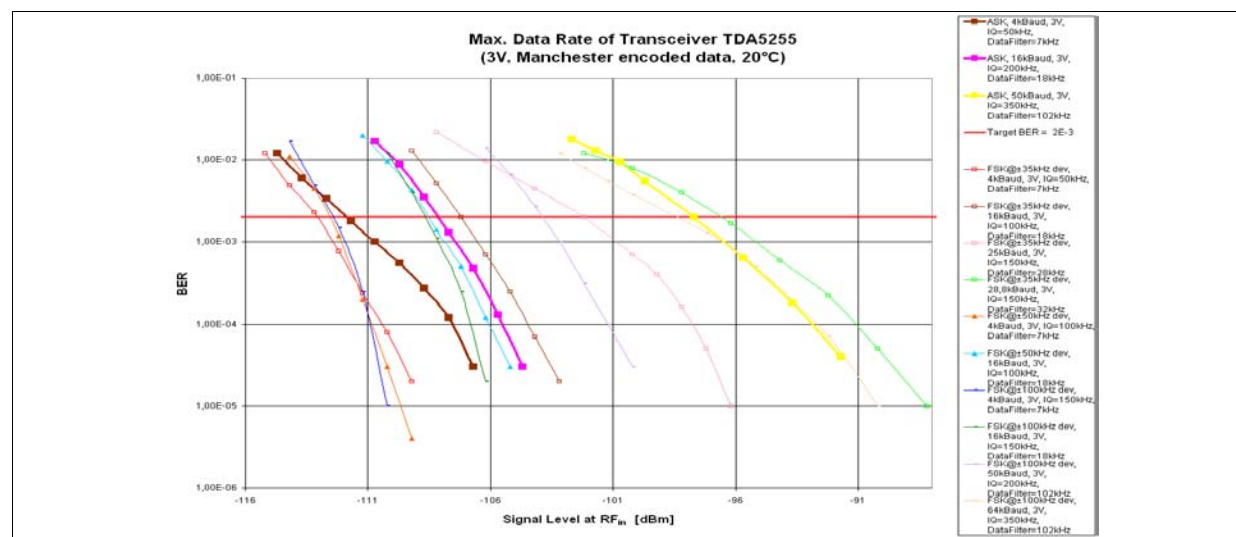
Figure 3-38 Datarates and Sensitivity
