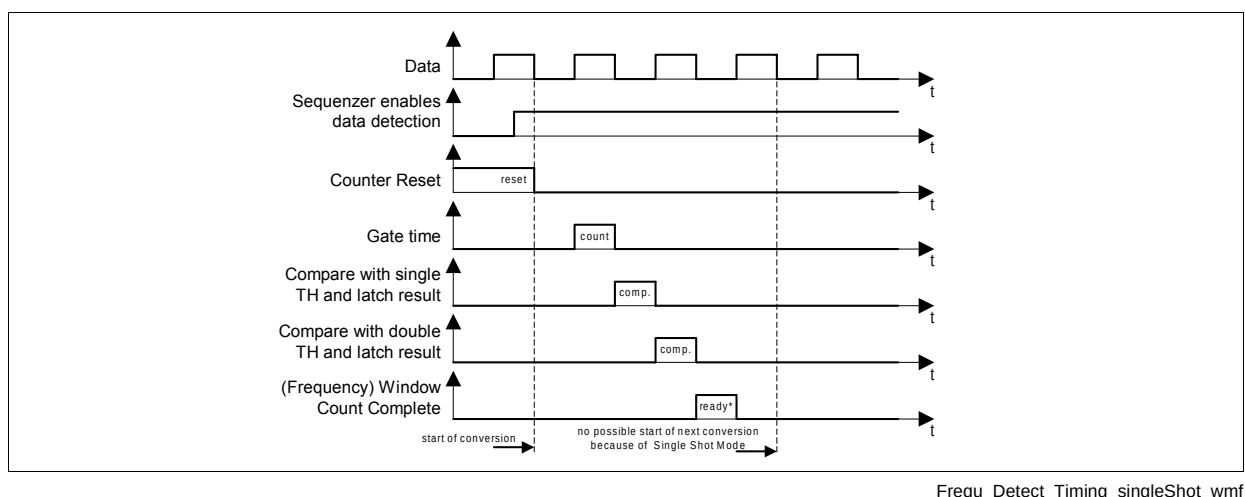
Figure 3-32 Frequency Detection timing in Single Shot mode
