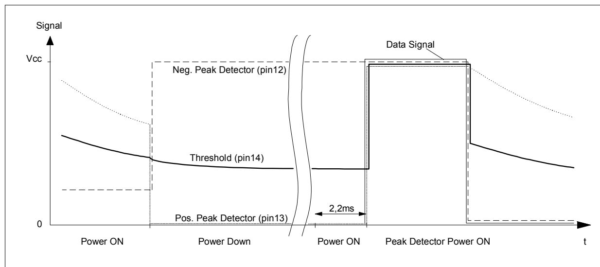
Figure 3-30 Power down mode
