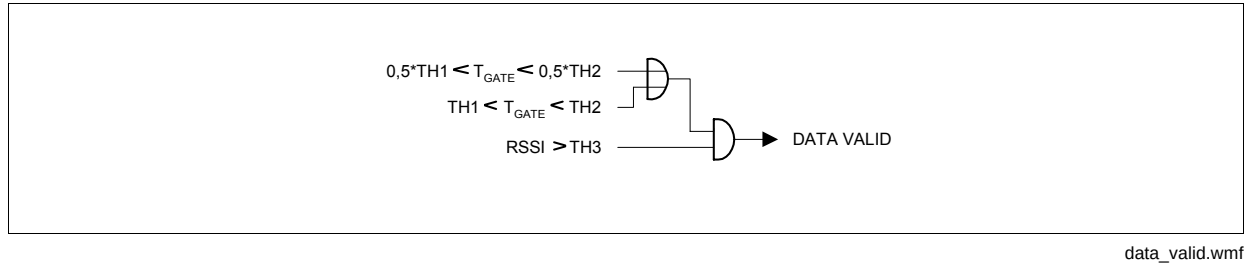
Figure 2-13 Data Valid Circuit
