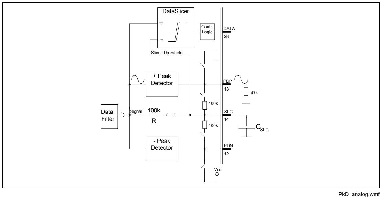
Figure 3-28 Peak Detector as analog Buffer (v=1)
