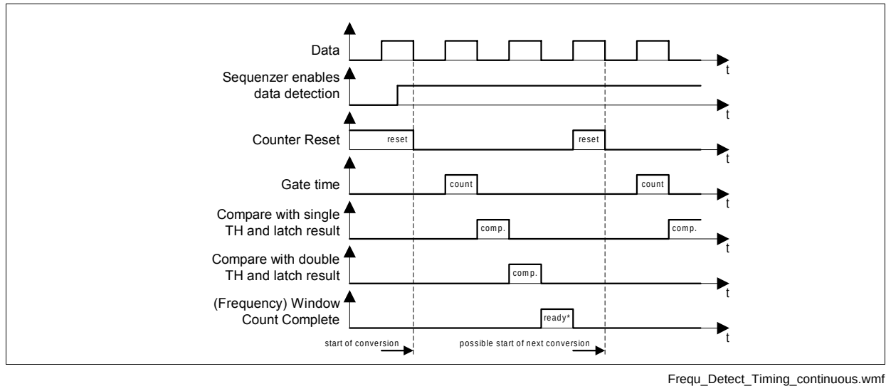
Figure 3-31 Frequency Detection timing in continuous mode
