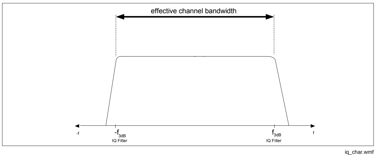
Figure 3-21 IQ Filter and frequency characteristics of the receive system
