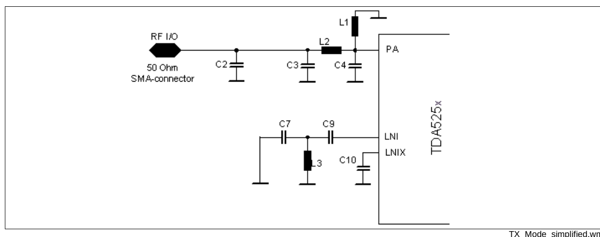
Figure 3-5 TX_Mode_simplified
