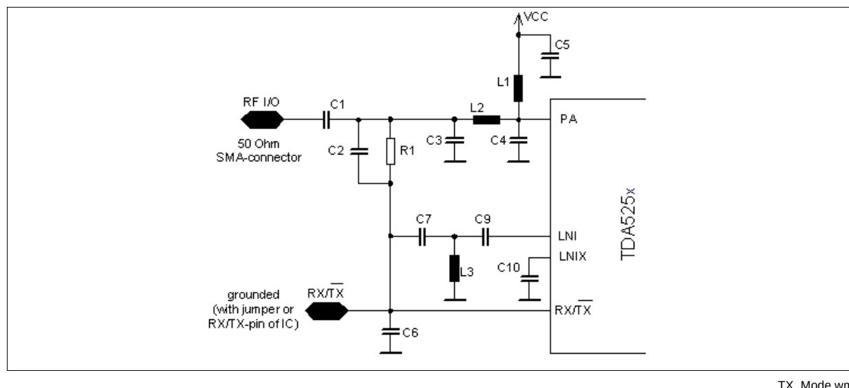
Figure 3-4 TX_Mode
