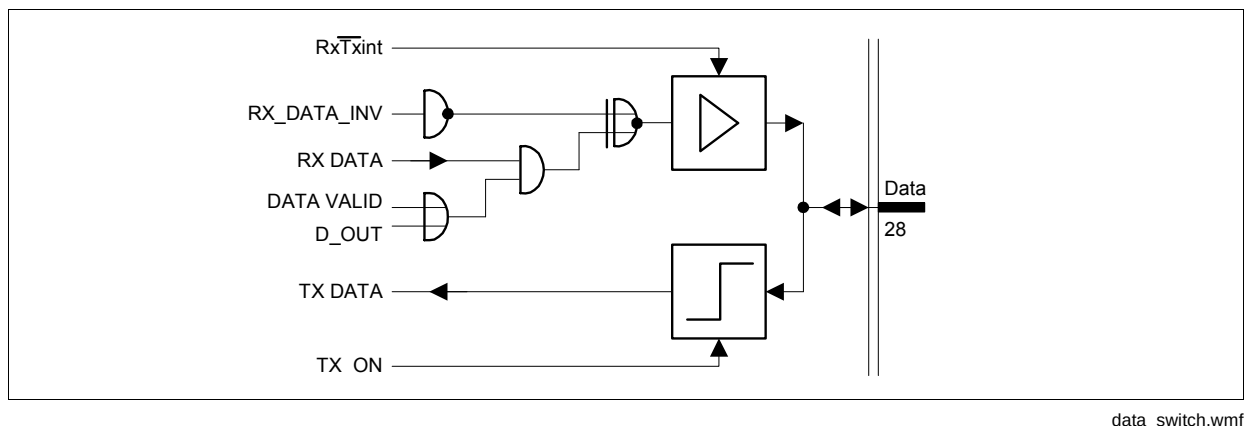
Figure 2-14 Data Input/Output Circuit
