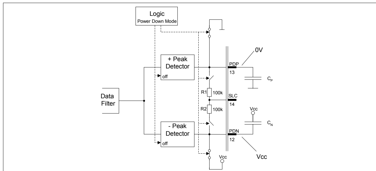
Figure 3-29 Peak detector - power down mode
