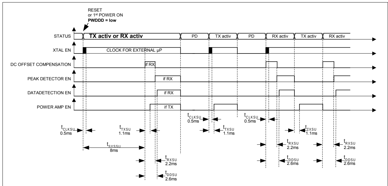
Figure 2-15 1 st start or reset in active mode
