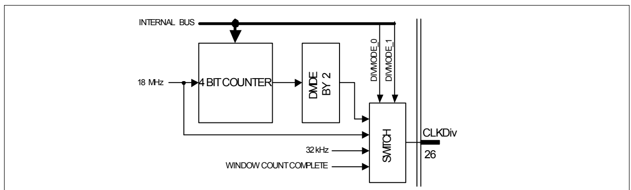
Figure 2-18 Clock Divider
