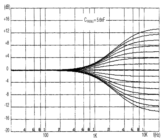
Figure 6: Treble response
