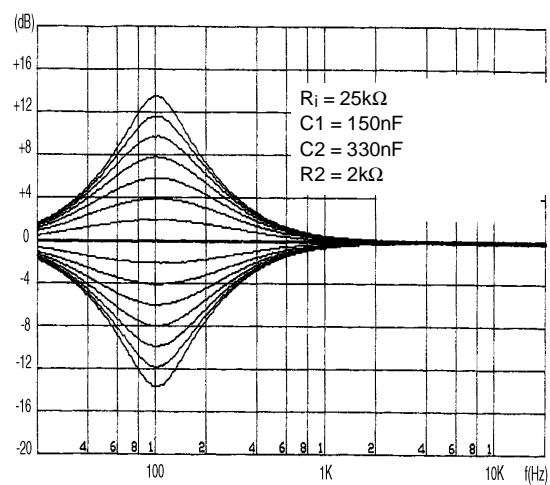
Figure 5: Bass response
