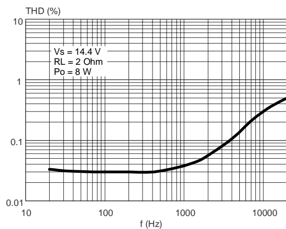
Figure 8. Distortion vs. Frequency ( 2\Omega )
