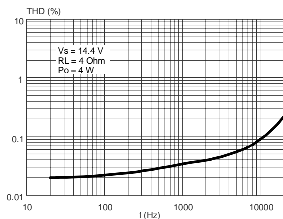
Figure 7. Distortion vs. Frequency ( 4\Omega )
