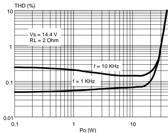
Figure 6. Distortion vs. Output Power ( 2\Omega )
