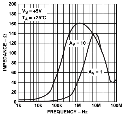
Figure 13. Closed-Loop Output Impedance vs. Frequency
