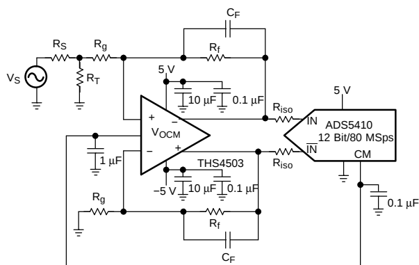
Using the THS4503 With the ADS5410
