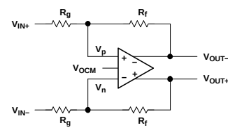
Diagram For Input Common-Mode Range Equations
