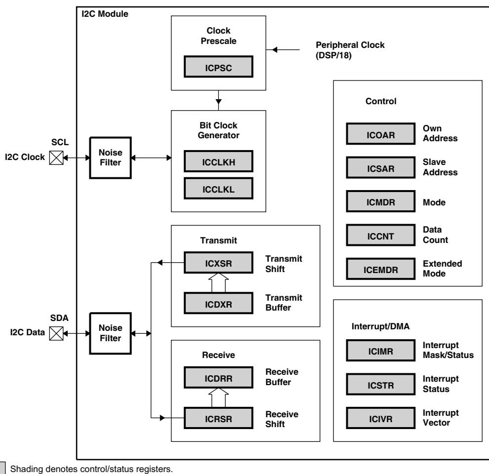
Figure 6-29. I2C Module Block Diagram
