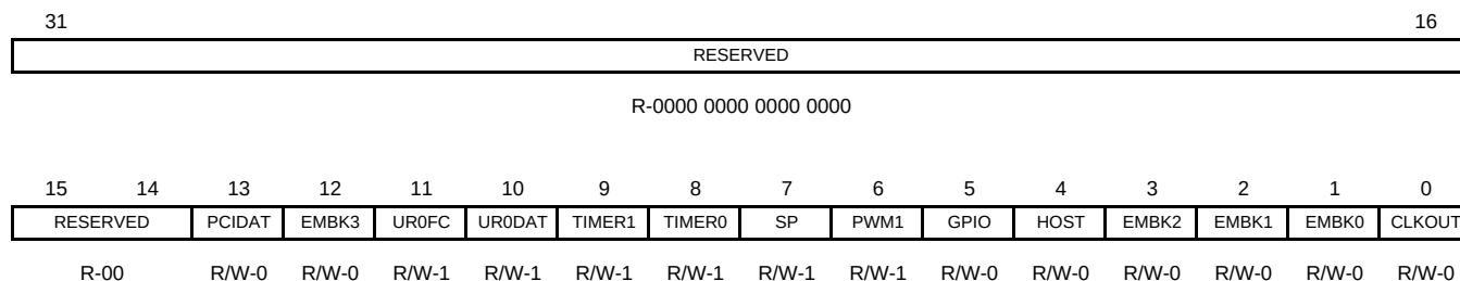
Figure 3-1. VDD3P3V_PWDN Register
