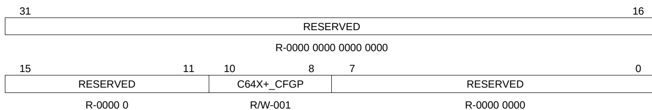
Figure 3-6. MSTPRI0 Register
