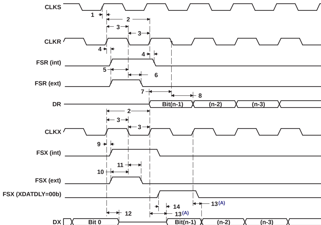
Figure 6-36. McBSP Timing (B)
