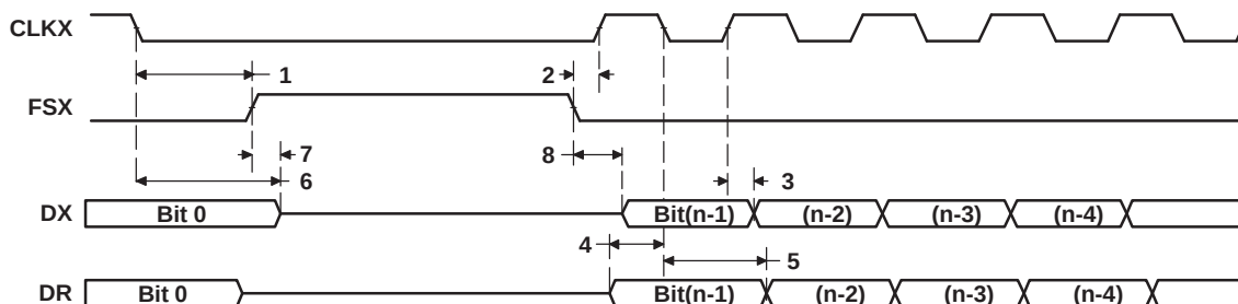
Figure 6-38. McBSP Timing as SPI Master or Slave: CLKSTP = 10b, CLKXP = 0
