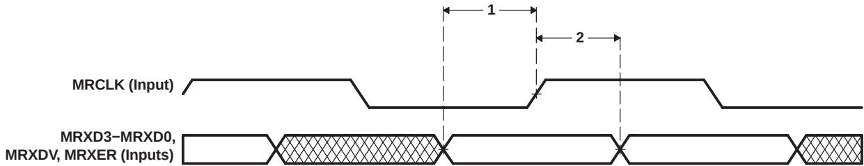
Figure 6-48. EMAC Receive Interface Timing
