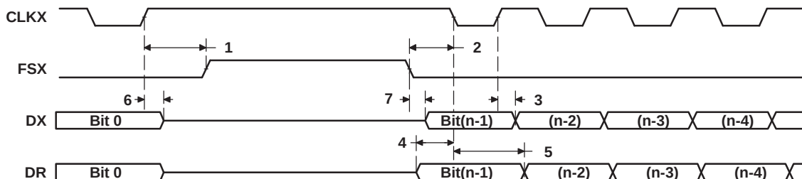
Figure 6-41. McBSP Timing as SPI Master or Slave: CLKSTP = 11b, CLKXP = 1
