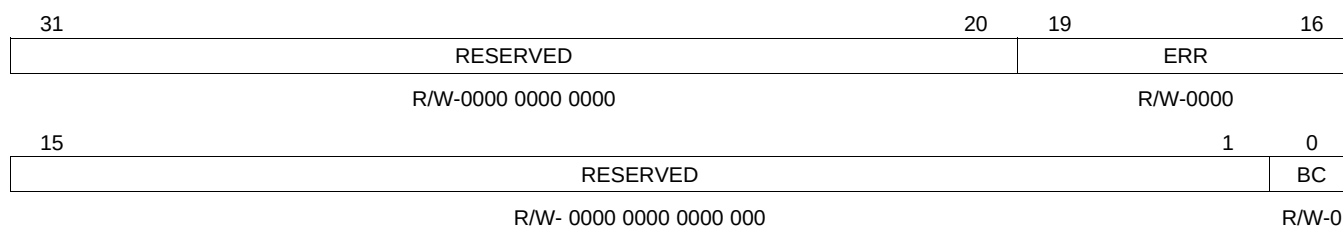
Figure 3-4. BOOTCMPLT Register
