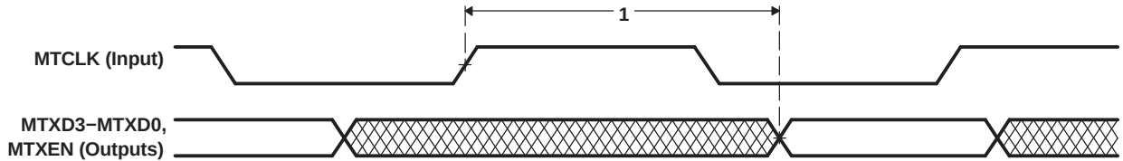
Figure 6-49. EMAC Transmit Interface Timing
