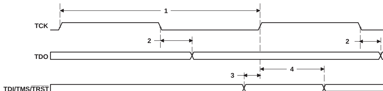
Figure 6-59. JTAG Test-Port Timing
