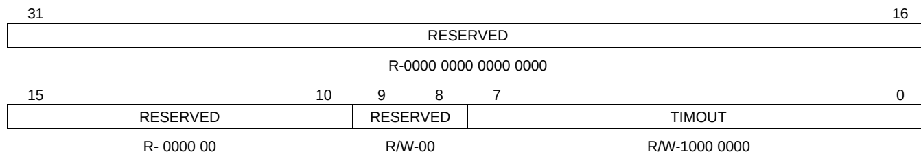
Figure 3-8. HPICTL Register
