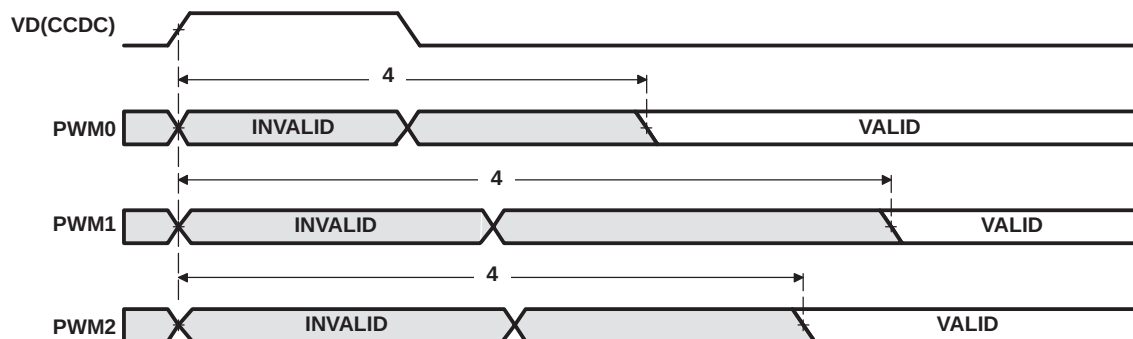
Figure 6-54. PWM Output Delay Timing
