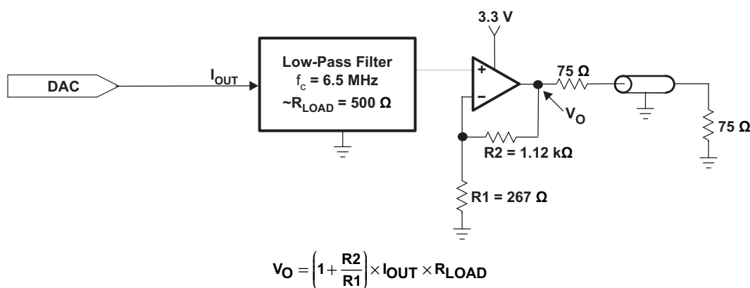
Figure 6-27. Typical Output Circuit for NTSC/PAL Video From DACs
