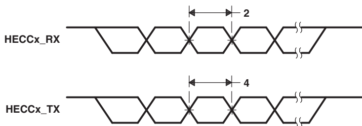
Figure 6-45. HECC Transmit/Receive Timing
