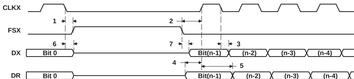
Figure 6-39. McBSP Timing as SPI Master or Slave: CLKSTP = 11b, CLKXP = 0
