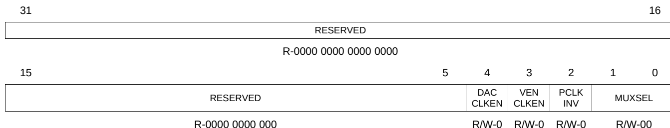
Figure 3-2. VPSS_CLKCTL Register
