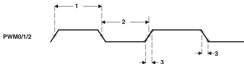
Figure 6-53. PWM Output Timing
