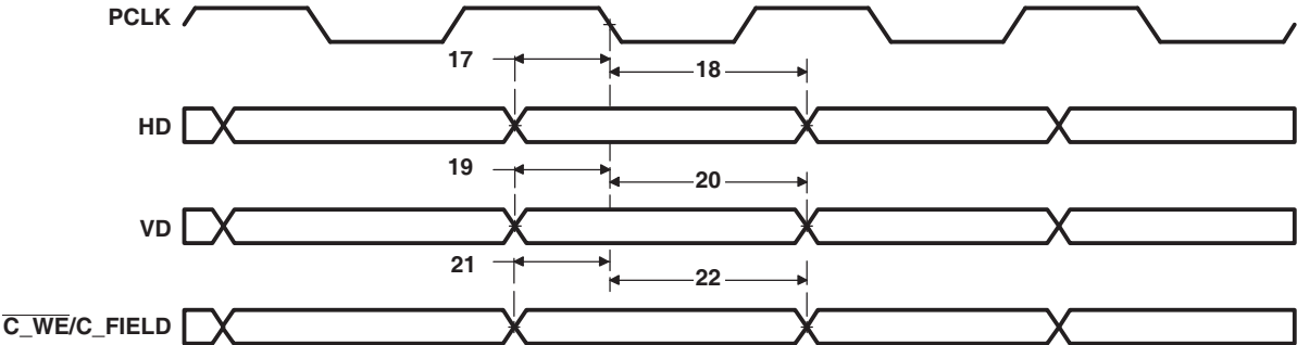
Figure 6-22. VPFE (CCD) Master Mode Control Output Data Timing
