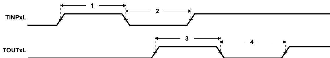
Figure 6-52. Timer Timing
