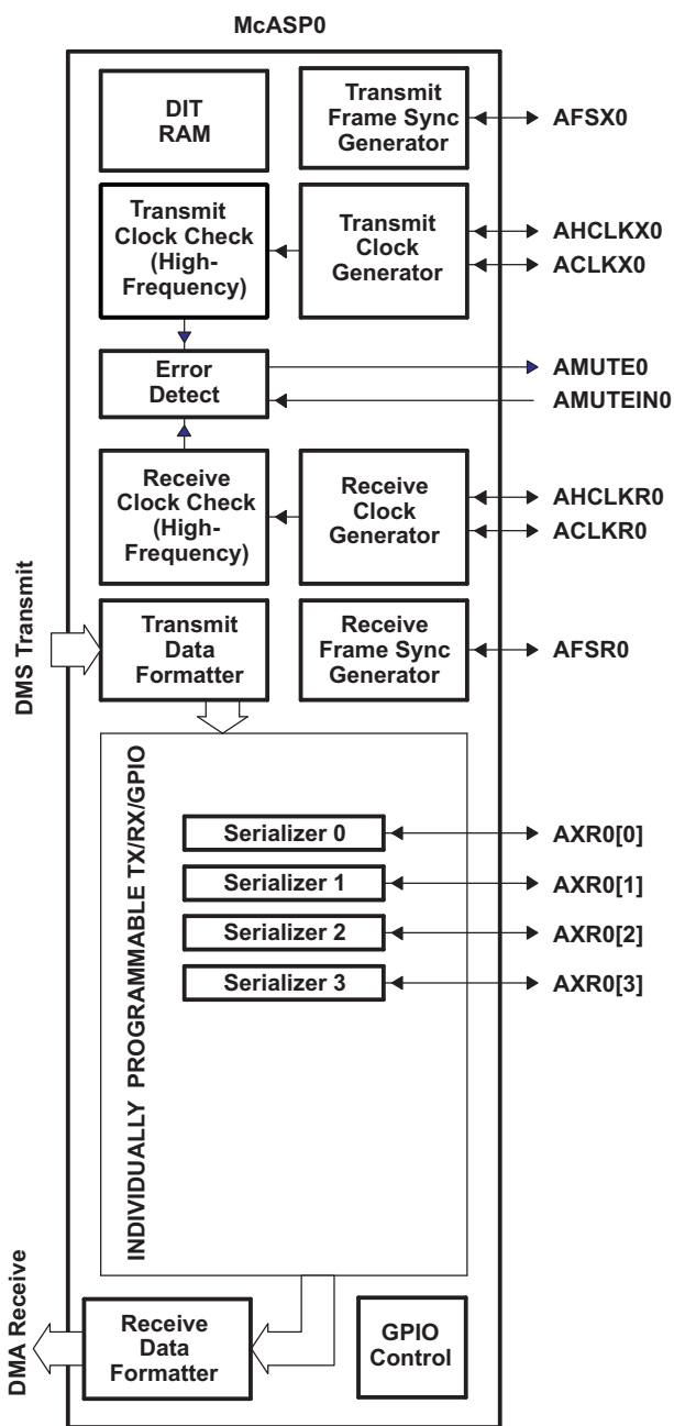
Figure 6-42. McASP0 Configuration
