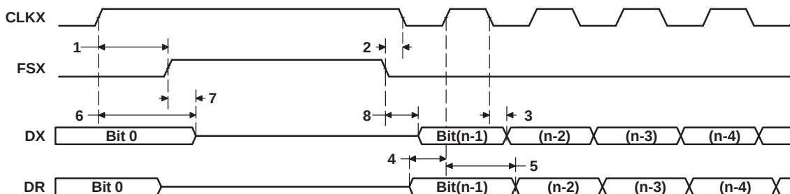
Figure 6-40. McBSP Timing as SPI Master or Slave: CLKSTP = 10b, CLKXP = 1
