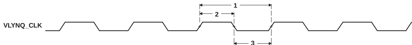
Figure 6-55. VLYNQ_CLK Timing for VLYNQ
