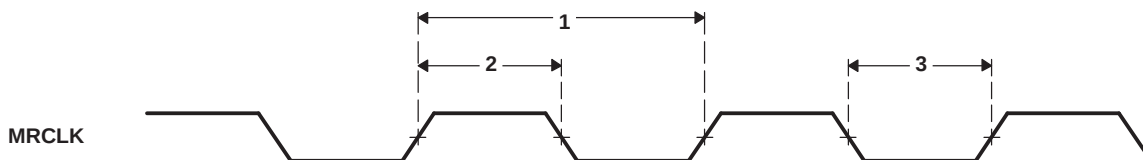
Figure 6-46. MRCLK Timing (EMAC - Receive)
