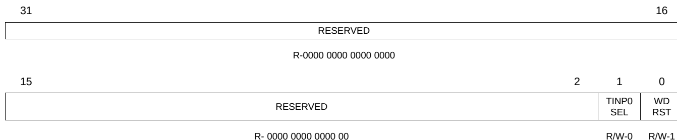
Figure 3-9. TIMERCTL Register
