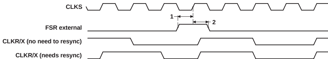
Figure 6-37. FSR Timing When GSYNC = 1
