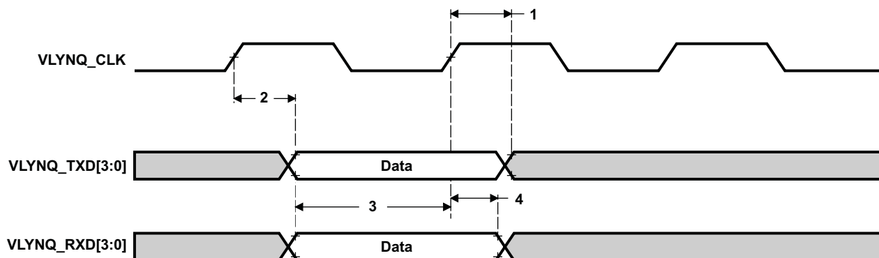
Figure 6-56. VLYNQ Transmit/Receive Timing
