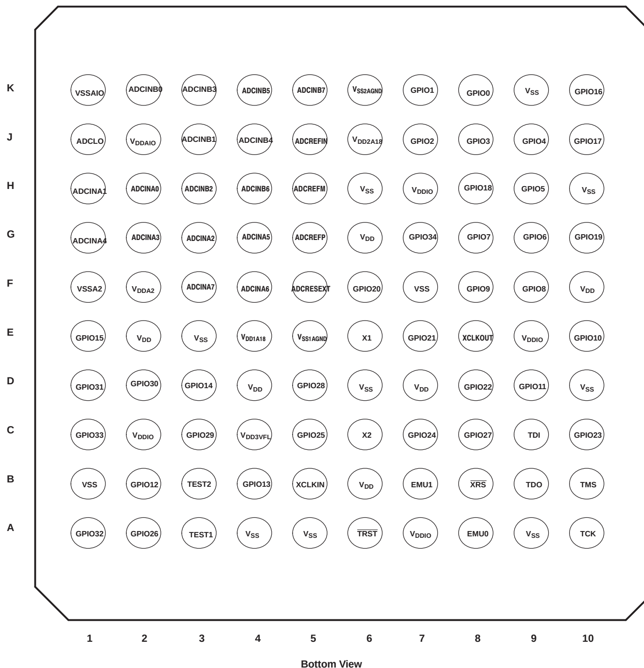
Figure 2-5. TMS320F2809, TMS320F2808, TMS320F2806, TMS320F2802, TMS320F2801, TMS320C2802, TMS320C2801 100-Ball GGM and ZGM MicroStar BGA™ (Bottom View)
