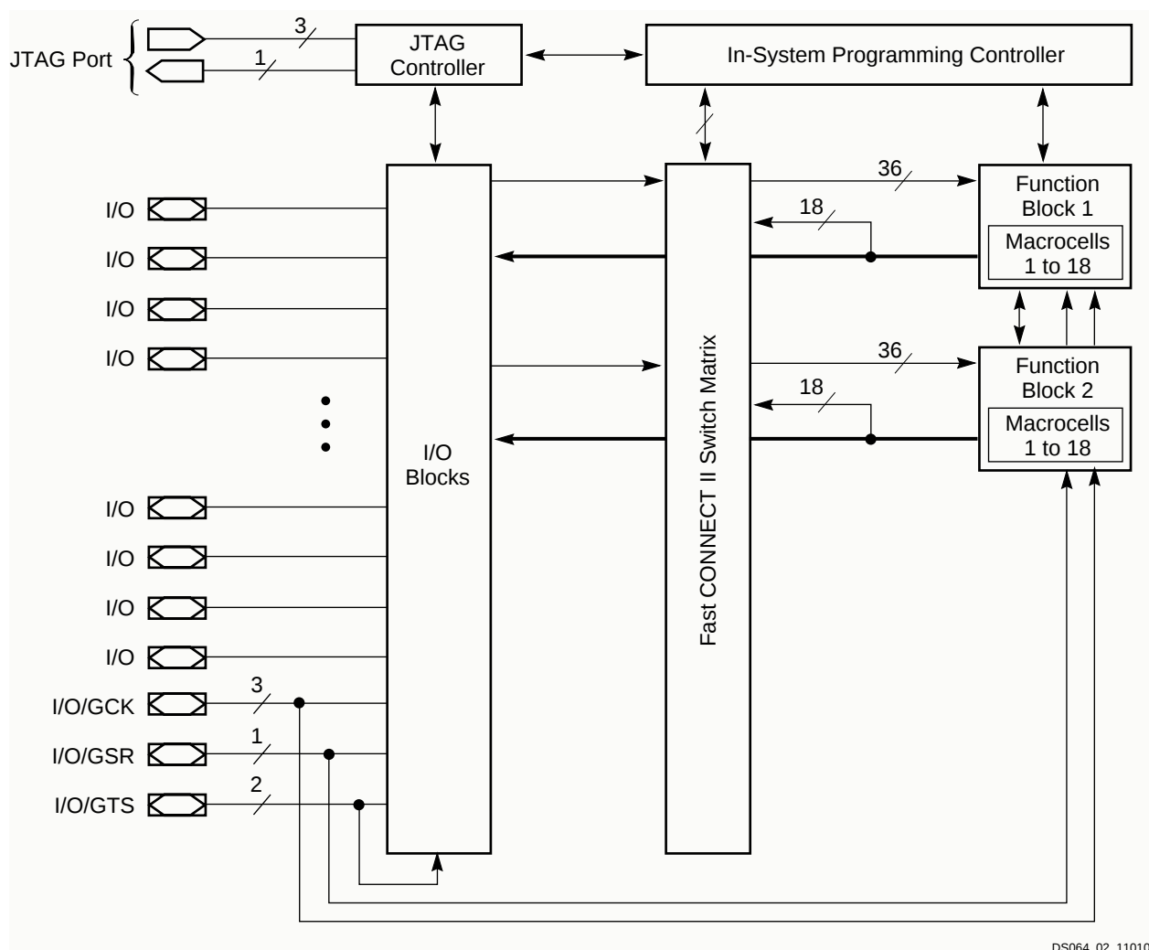
Figure 2: XC9536 Architecture
