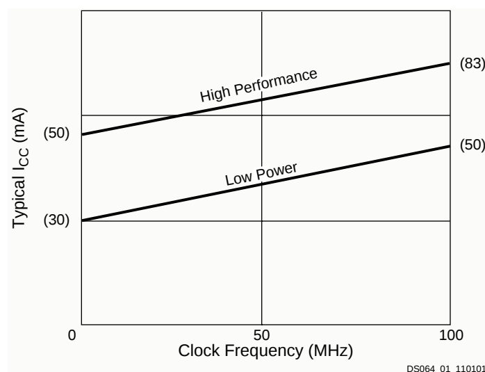
Figure 1: Typical I_{CC} vs. Frequency for XC9536
