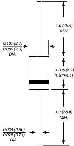
DO-41
