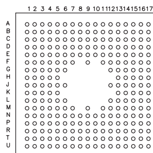
Figure 4-2. 256-ball BGA Pinout (Top View)
