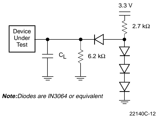
Figure 9. Test Setup
