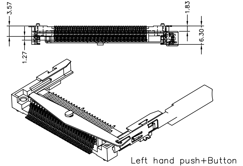
Dimension L
