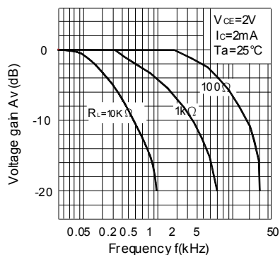
Fig. 10 Frequency Response
