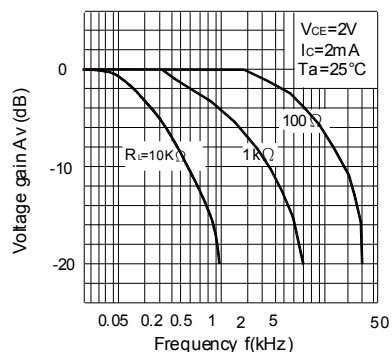
Fig. 10 Frequency Response
