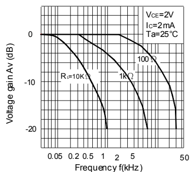
Fig. 10 Frequency Response
