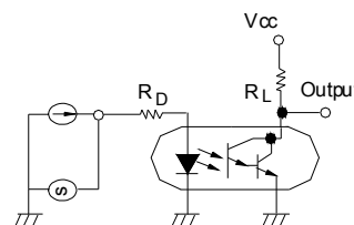
Test Circuit for Frequency Response
