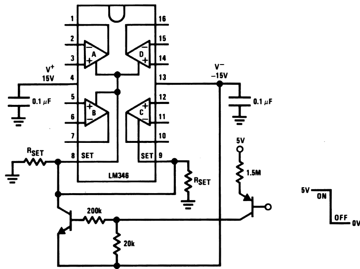
Circuit Shutdown
