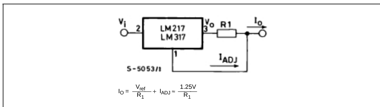
Figure 7 : Current Regulator
