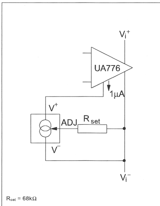
Figure 7 : Micropower Bias
