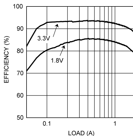
\eta vs Load "X" V_{in} = 5V , V_o = 1.8V & 3.3V
