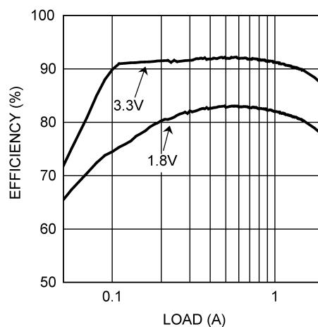
\eta vs Load "Z" V_{in} = 5V , V_o = 3.3V & 1.8V
