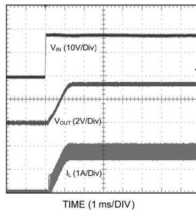
Power Up ( V_{OUT} = 3.3V , 1.5A Loaded)
