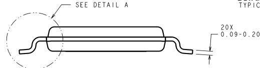
20-Lead Plastic eTSSOP Package NS Package Number MXA20A
