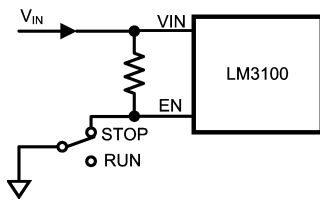
FIGURE 1. Shutdown Implementation
