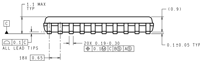
20-Lead Plastic eTSSOP Package NS Package Number MXA20A
