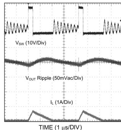
Discontinuous Mode Operation ( V_{OUT} = 3.3V , 1.5A Loaded)
