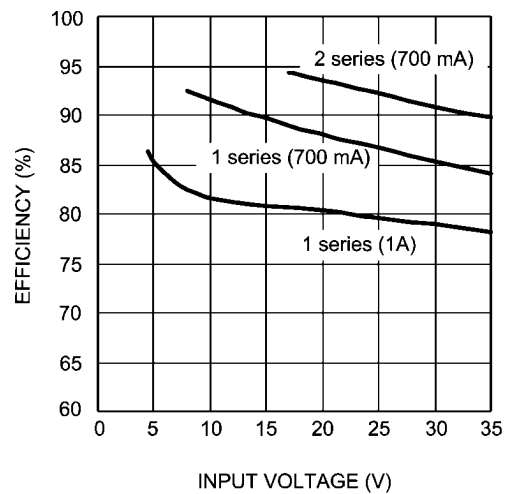
700 mA and 1A Efficiency
