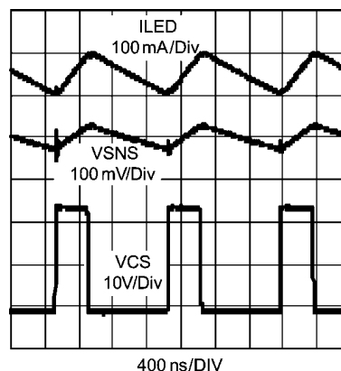
FIGURE 2. Hysteretic Switching Waveforms
