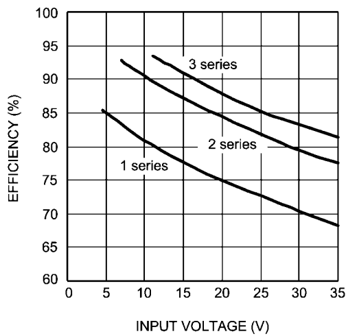
350 mA Efficiency
