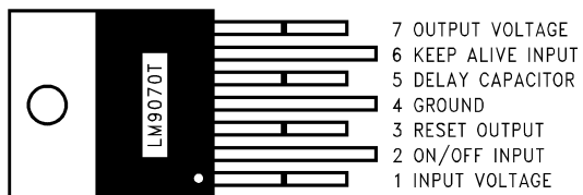
7-Lead TO-220 Package (Odd numbered pins bent forward away from package body)
