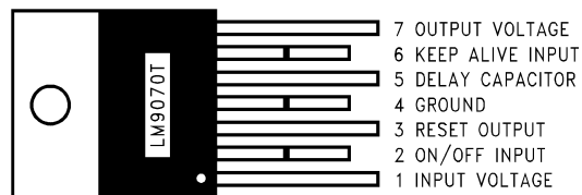
7-Lead TO-220 Package (Even numbered pins bent forward away from package body)
