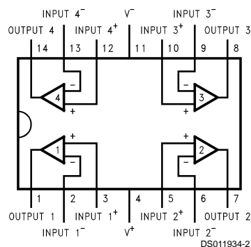
14-Pin DIP/SO
