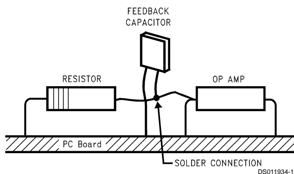
FIGURE 5. Air Wiring
