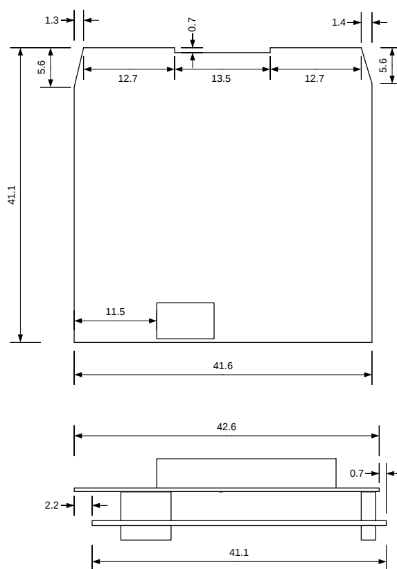
Digital Board
