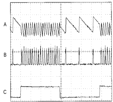
LOAD-TRANSIENT RESPONSE
