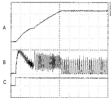
POWER-UP RESPONSE
