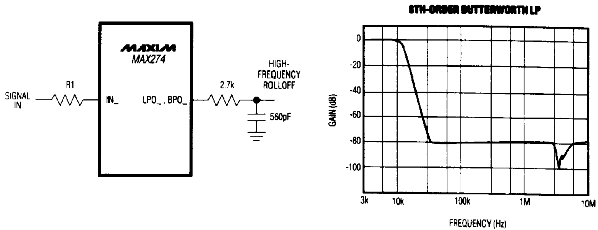
Figure 10. External RC Lowpass for High-Frequency Roll-off
