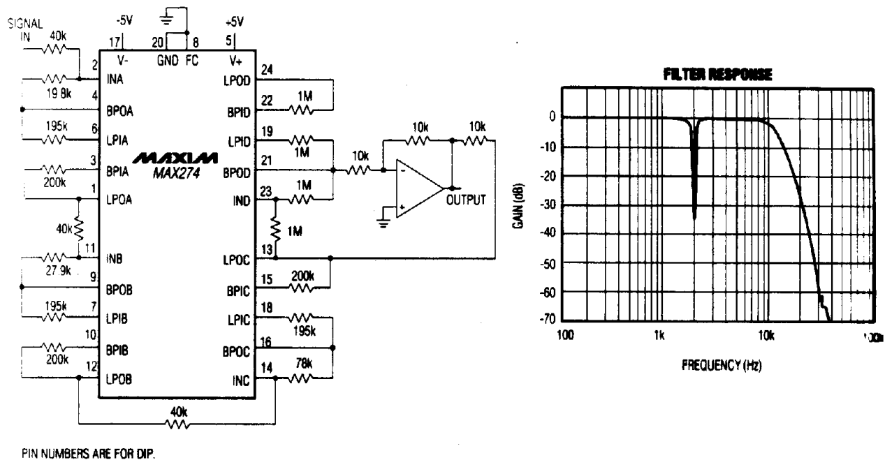
Figure 11. 10kHz 6th-Order Butterworth Lowpass Filter with 2kHz Notch (MAX274)
