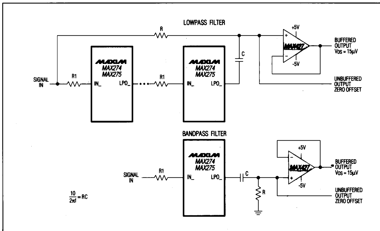
Figure 8b. Trimless Offset Removal
