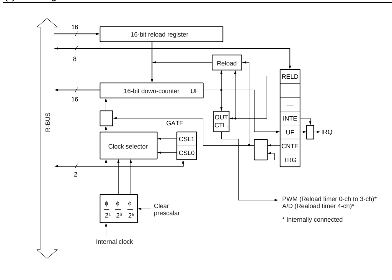
(2) Block diagram
