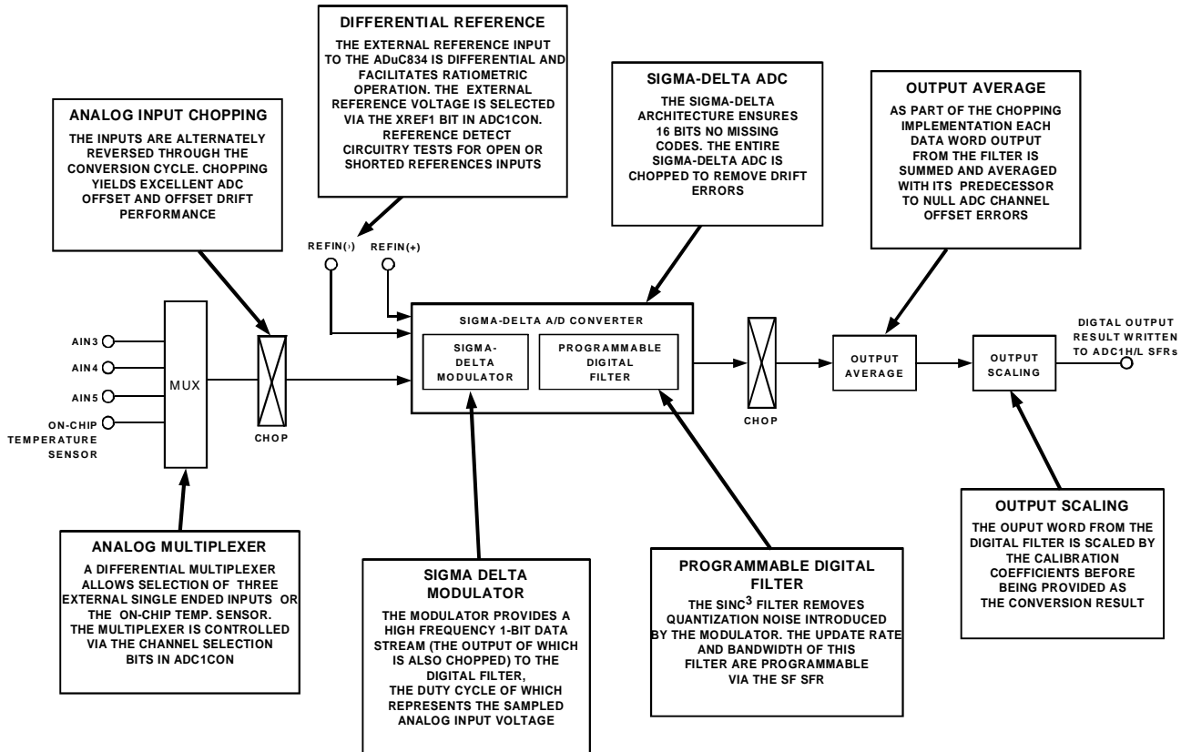
Figure 8. Auxiliary ADC Block Diagram
