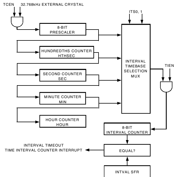
Figure 33. TIC, Simplified Block Diagram
