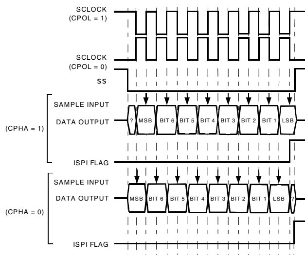
Figure 34. ADuC834, SPI Timing, All Modes
