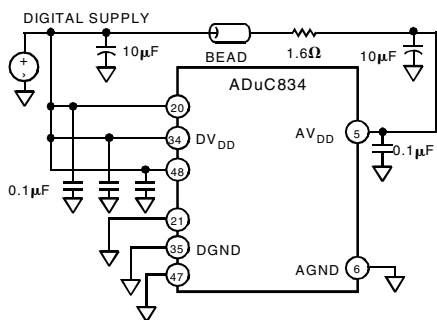
Figure 49. External Single Supply Connections
