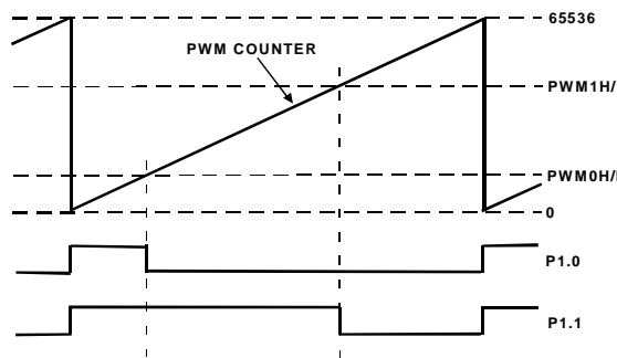
Figure 29. PWM Mode 3
