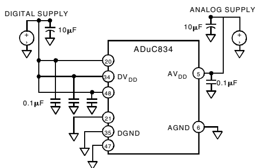
Figure 48. External Dual Supply Connections
