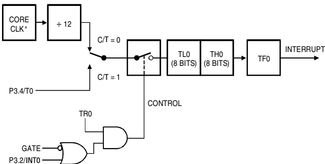
Figure 36. Timer/Counter 0, Mode 1
