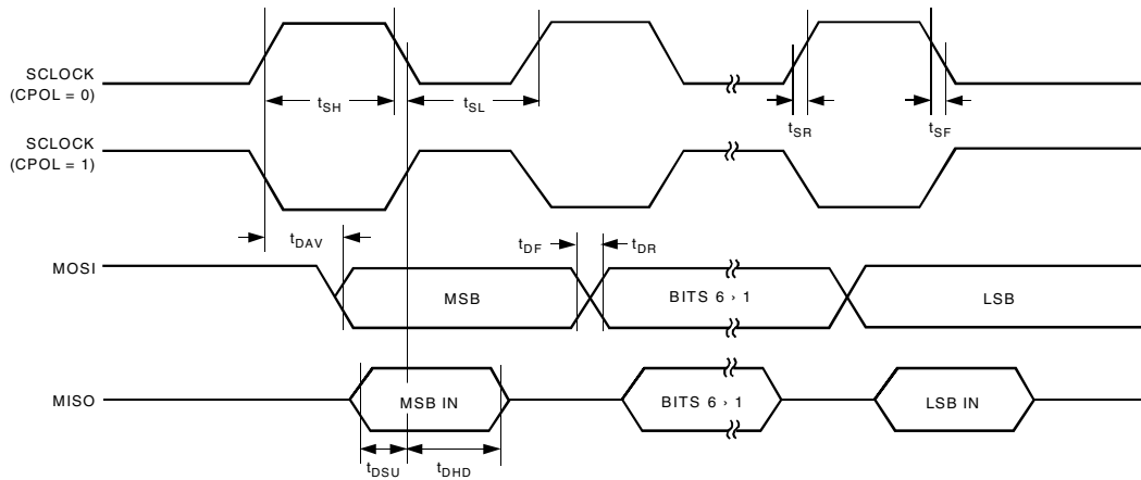
Figure 60. SPI Master Mode Timing (CPHA = 1)
