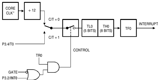
Figure 35. Timer/Counter 0, Mode 0
