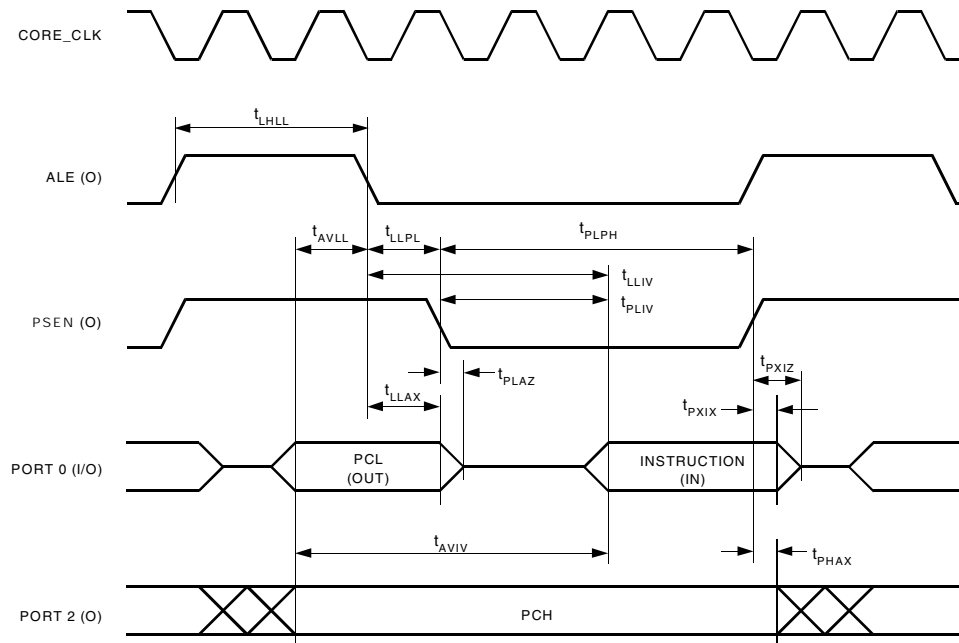
Figure 56. External Program Memory Read Cycle
