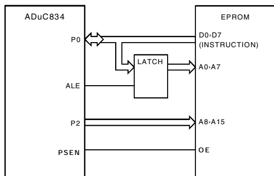
Figure 45. External Program Memory Interface
