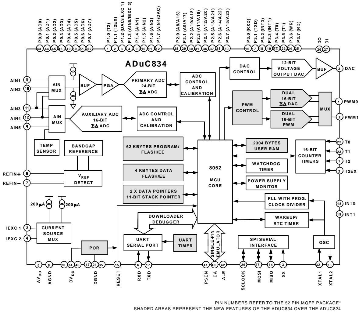
Figure 1. ADuC834 Detailed Block Diagram
