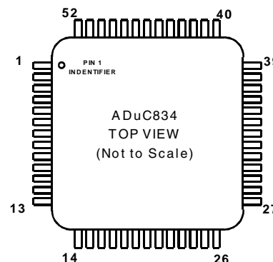
52-Lead CSP
