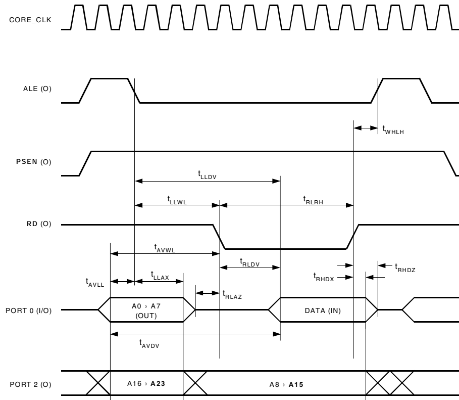
Figure 57. External Data Memory Read Cycle
