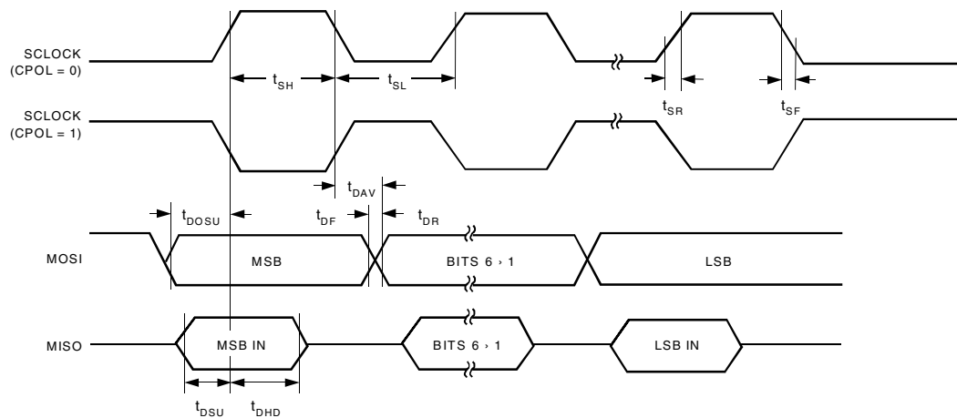
Figure 61. SPI Master Mode Timing (CPHA = 0)
