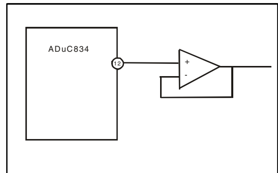
Figure 25. Buffering the DAC output
