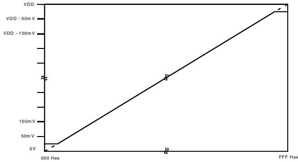
Figure 22. Endpoint Non-linearities due to Amplifier Saturation.
