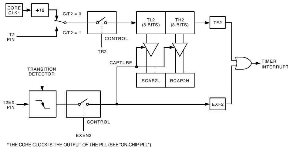
Figure 40. Timer/Counter 2, 16-Bit Capture Mode
