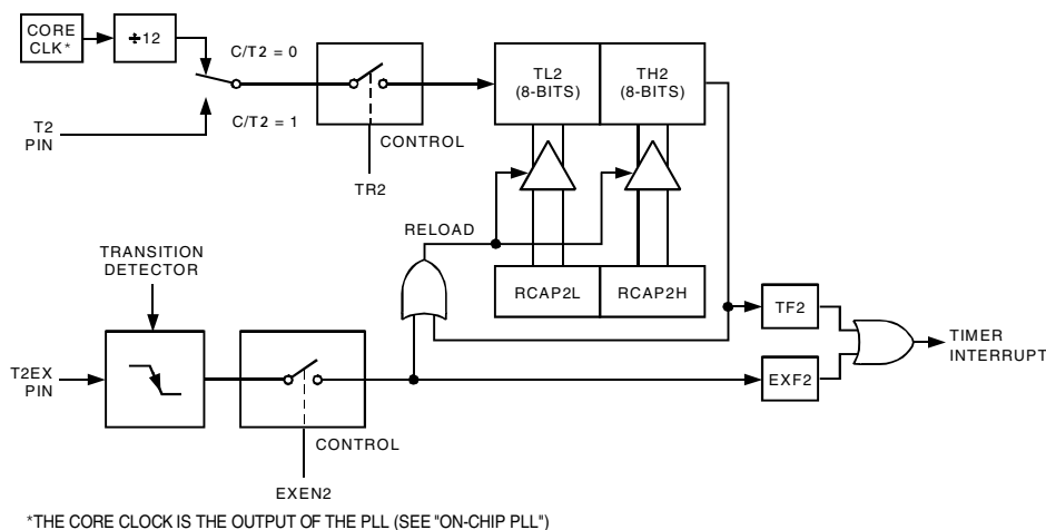
Figure 39. Timer/Counter 2, 16-Bit Autoreload Mode
