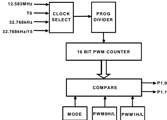
Figure 26. PWM Block Diagram
