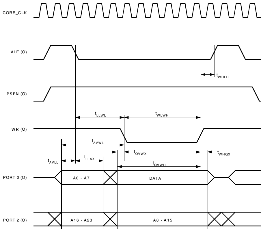
Figure 58. External Data Memory Write Cycle
