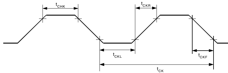
Figure 54. XTAL1 Input
