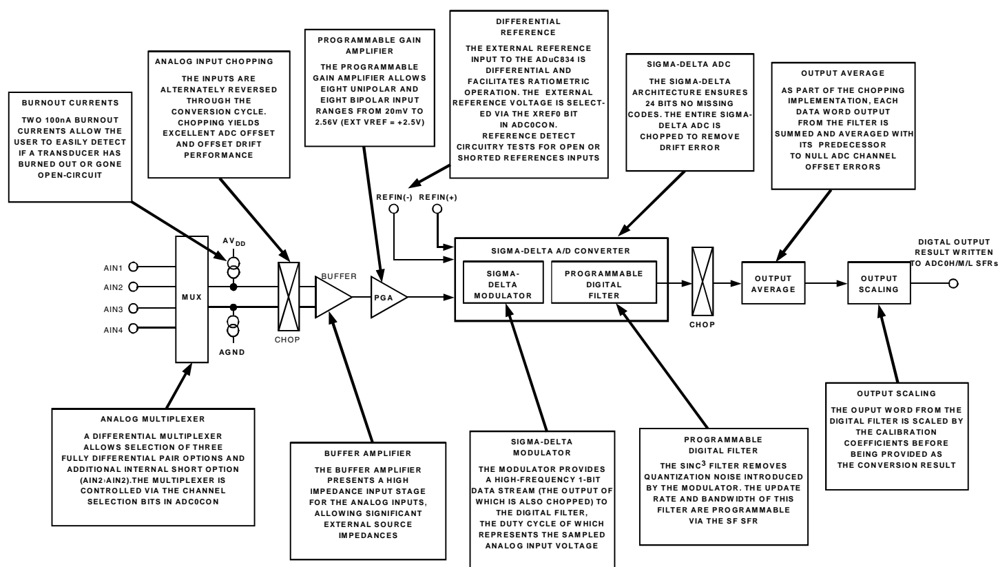
Figure 7. Primary ADC Block Diagram
