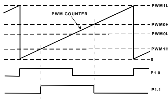
Figure 28. PWM Mode 2
