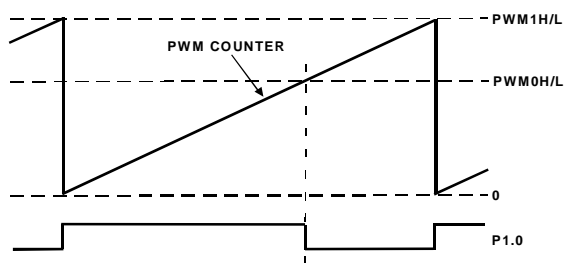
Figure 27. ADuC834 PWM in Mode 1
