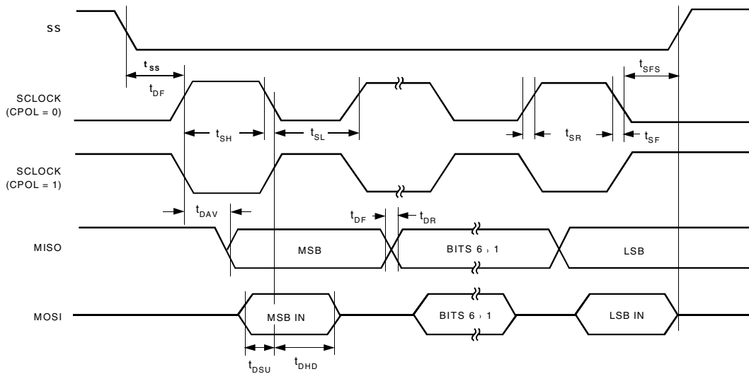
Figure 62. SPI Slave Mode Timing (CPHA = 1)
