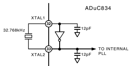
Figure 52. External Parallel Resonant Crystal Connections
