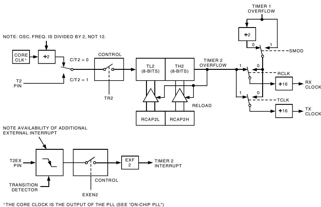
Figure 43. Timer 2, UART Baud Rates
