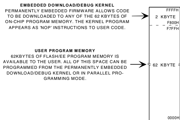
Figure 17. Flash/EE Program Memory Map in NORMAL mode
