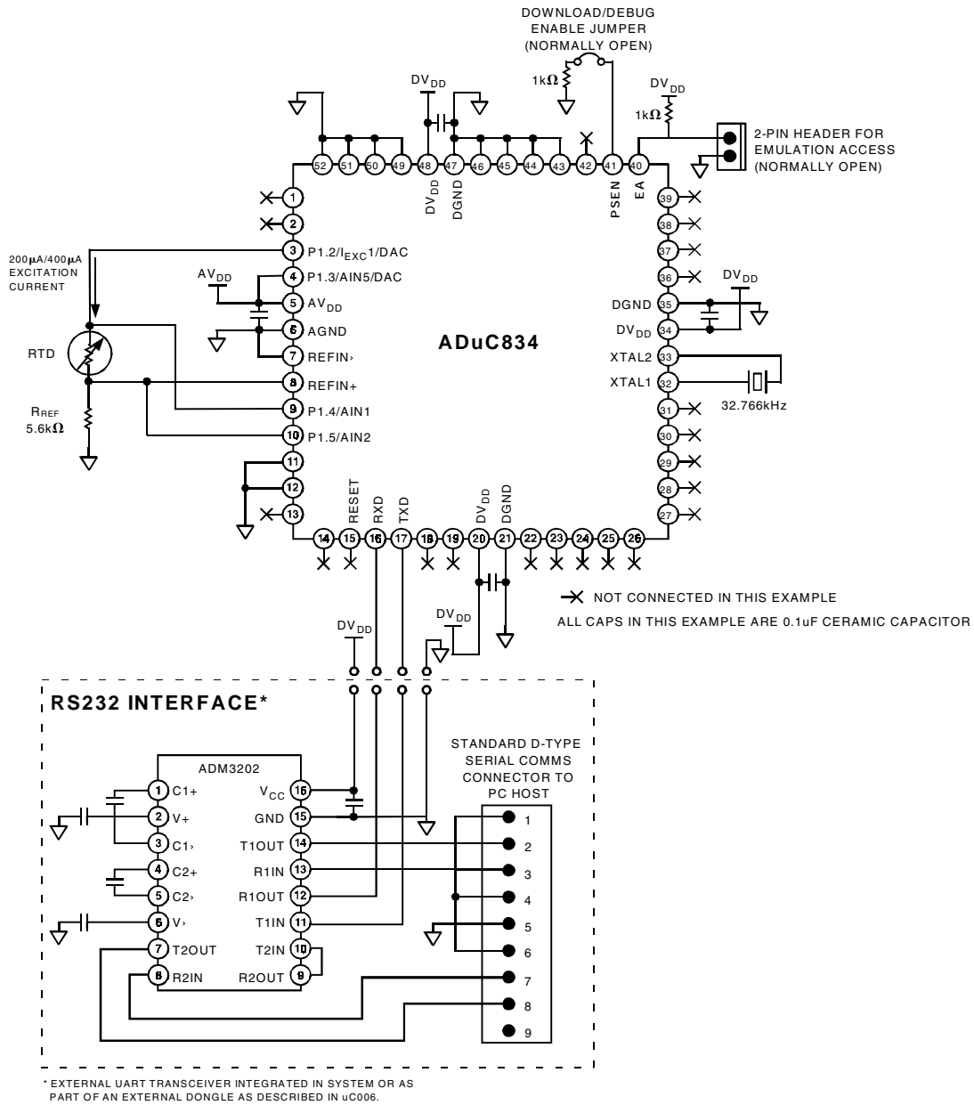
Figure 53. Typical System Configuration
