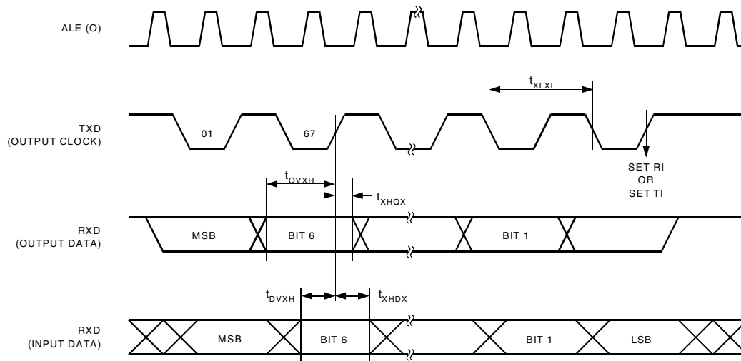
Figure 59. UART Timing in Shift Register Mode
