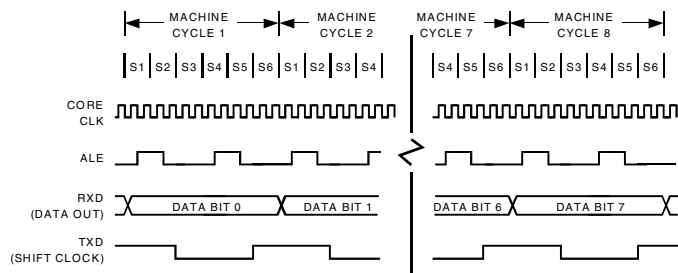
Figure 41. UART Serial Port Transmission, Mode 0.
