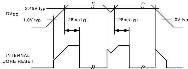
Figure 50. ADuC834 Internal Power-on-Reset operation
