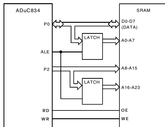
Figure 47. External Data Memory Interface (16 M Bytes Address Space)
