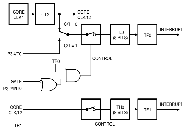
Figure 38. Timer/Counter 0, Mode 3
