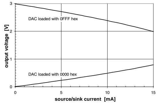
Figure 24. Source & Sink Current Capability with V_{REF} = V_{DD} = 3V
