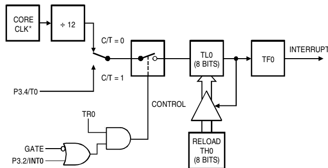
Figure 37. Timer/Counter 0, Mode 2
