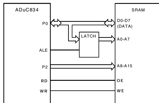
Figure 46. External Data Memory Interface (64kBytes Address Space)
