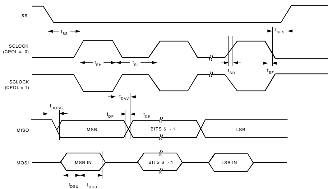
Figure 63. SPI Slave Mode Timing (CPHA = 0)
