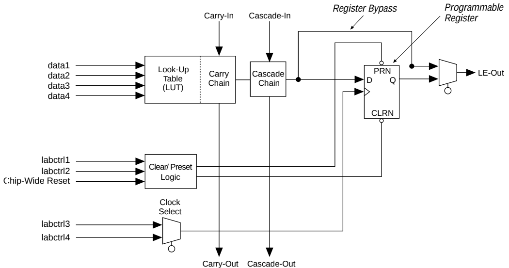
Figure 4. Logic Element
