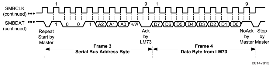
(d) Typical Pointer Set Followed by Immediate Read of a 1-Byte Register.
