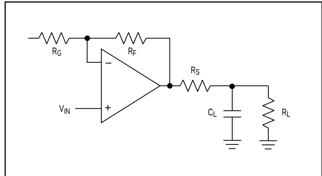
Figure 7a. Using an Isolation Resistor ( R_S ) for High Capacitive Loads
