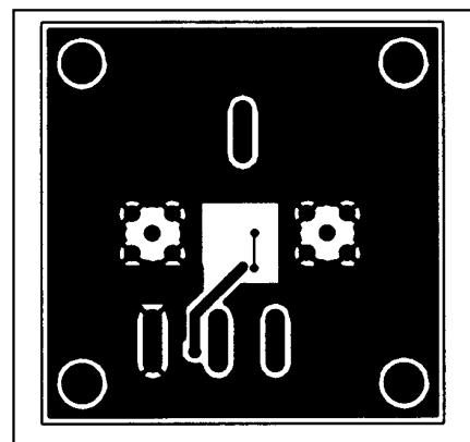
Figure 2c. High-Speed EV Board Layout—Solder Side
