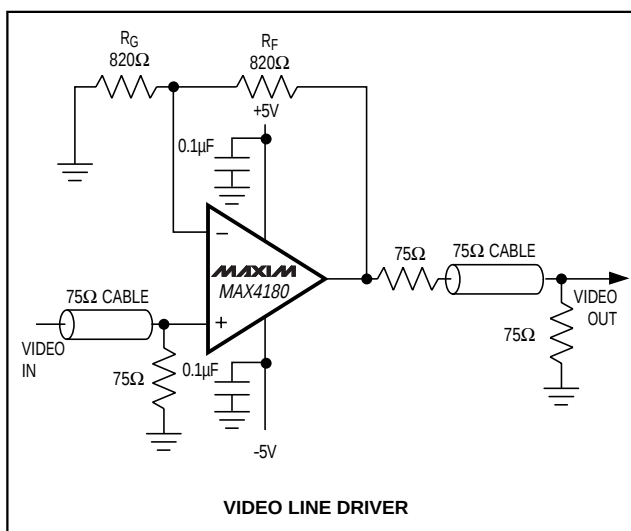
Figure 6. Video Line Driver
