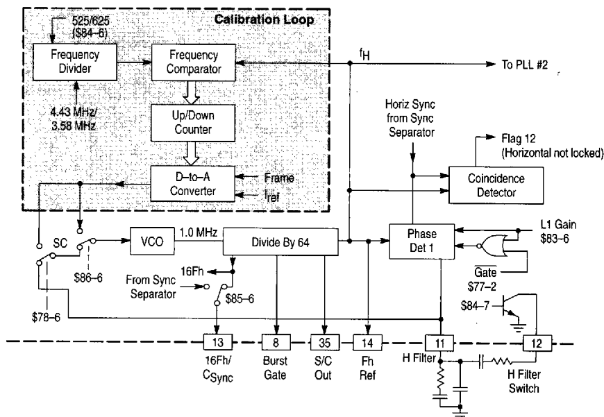
Figure 38. Horizontal PLL (PLL1)
