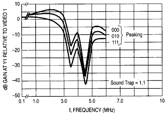
Figure 2. Composite Video Mode
