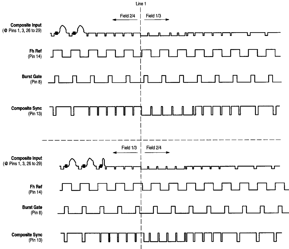
Figure 31. Horizontal Outputs versus Fields (PAL System)
