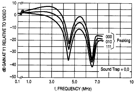
Figure 10. Composite Video Mode
