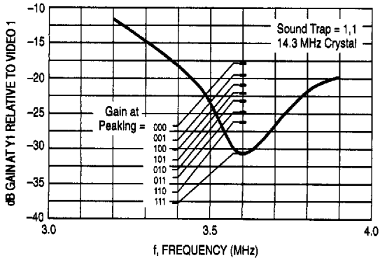
Figure 12. (3.58 MHz) Chroma Notch
