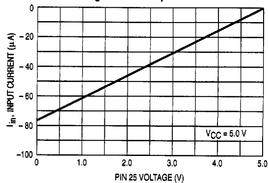
Figure 24. FC Input Current
