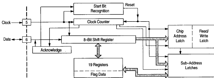
Figure 41. I 2 C Bus Interface and Decoder
