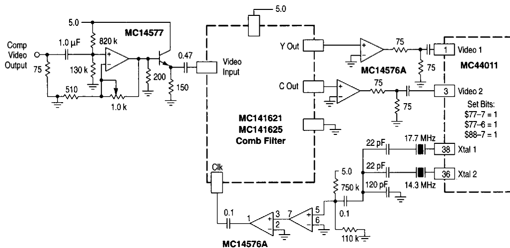
Figure 48. Implementing the Comb Filter
