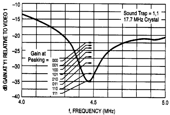
Figure 13. (4.43 MHz) Chroma Notch
