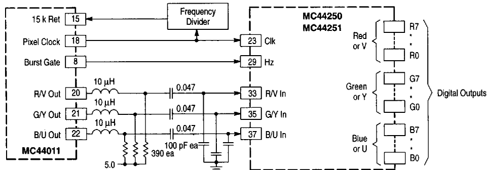
Figure 47. Connecting to a Triple A/D Converter
