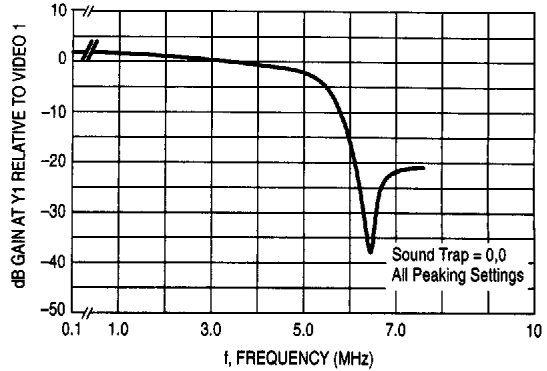
Figure 11. S-VHS Mode
