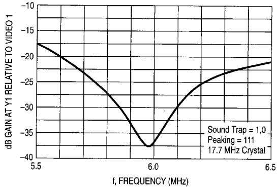
Figure 20. Composite Video Mode
