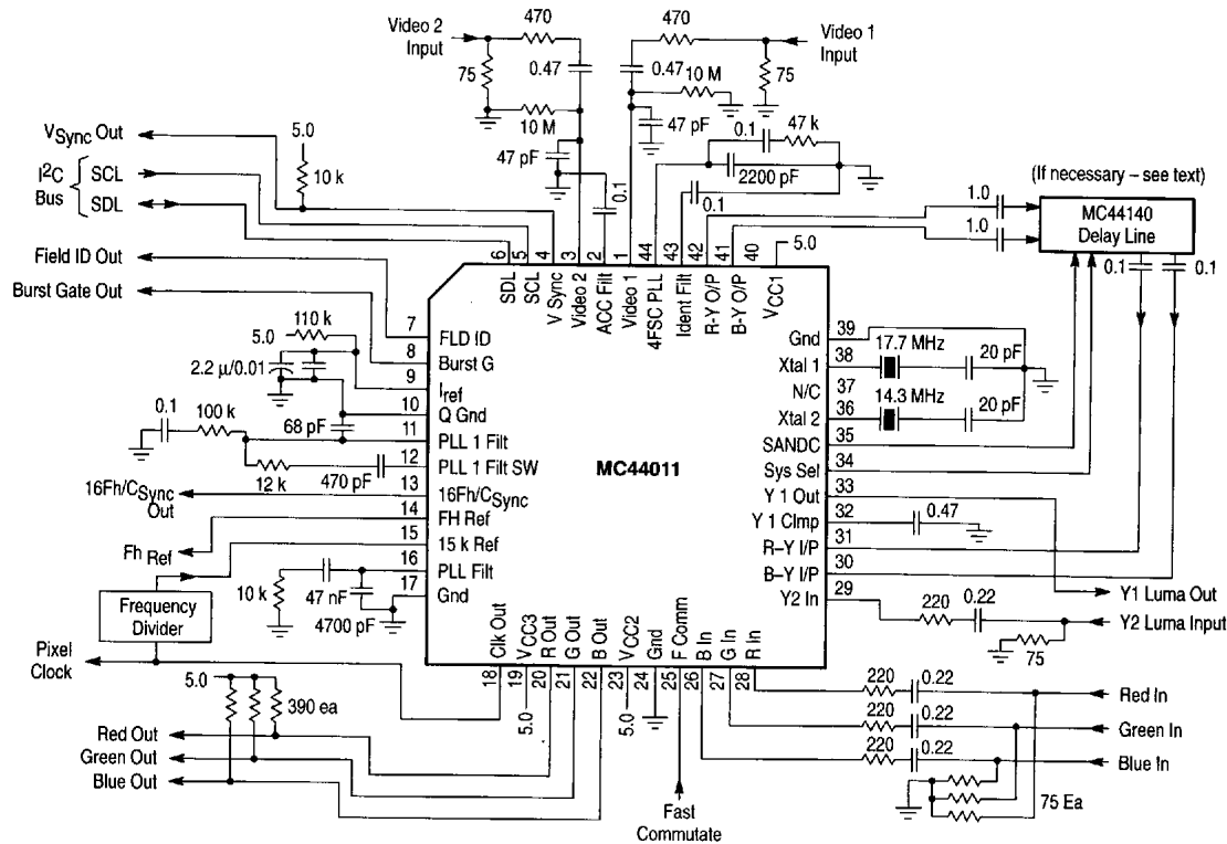
Figure 42. Basic Functional Circuit
