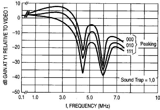
Figure 8. Composite Video Mode
