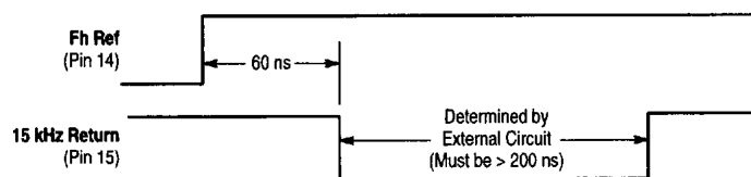
Figure 32. Horizontal PLL2 Timing
