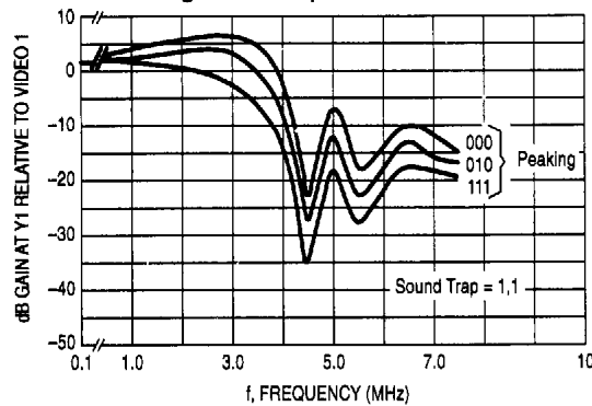
Figure 6. Composite Video Mode
