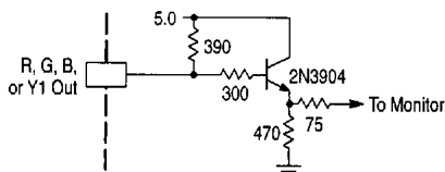
Figure 43. Output Buffer
