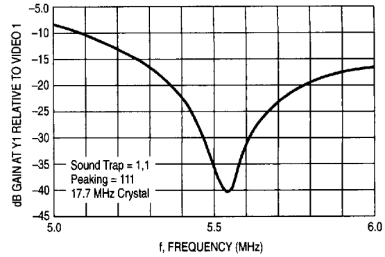
Figure 17. S-VHS Mode
