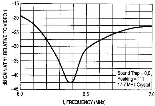
Figure 22. Composite Video Mode
