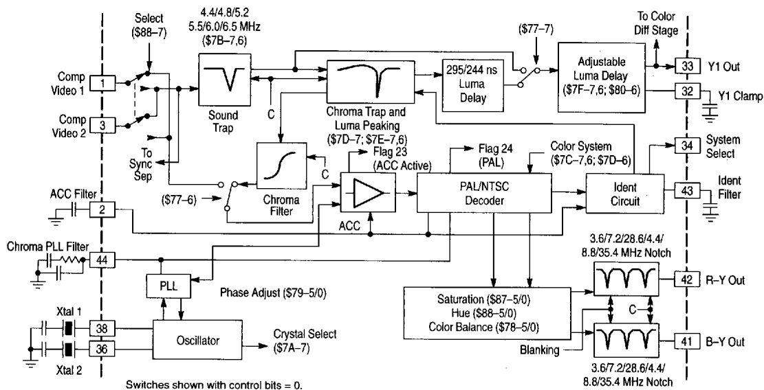
Figure 35. PAL/NTSC/S-VHS Decoder Block Diagram
