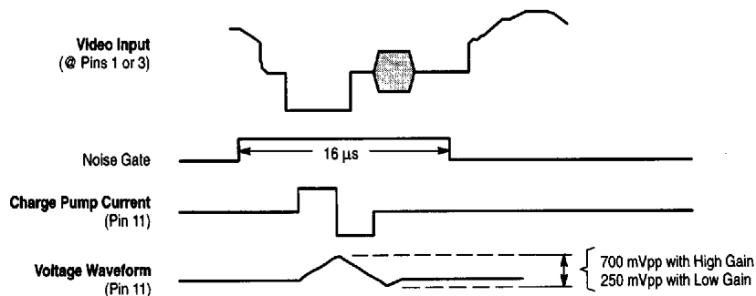
Figure 26. Horizontal PLL1 Noise Gate and Filter Pin
