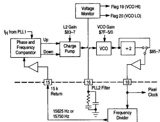
Figure 39. Pixel Clock PLL (PLL2)
