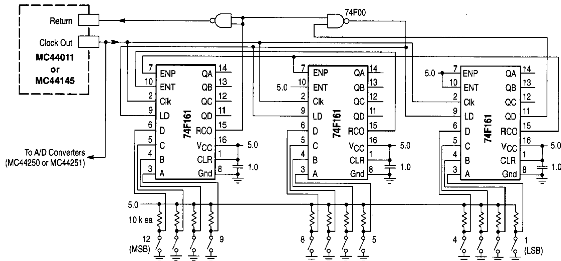
Figure 46. Suggested Frequency Divider
