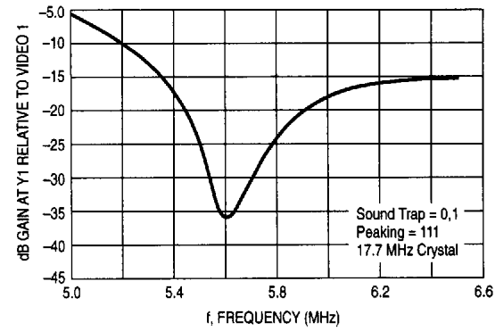
Figure 19. S-VHS Mode
