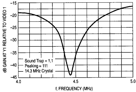
Figure 14. Composite Video Mode
