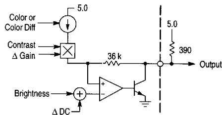
Figure 37. Output Stage
