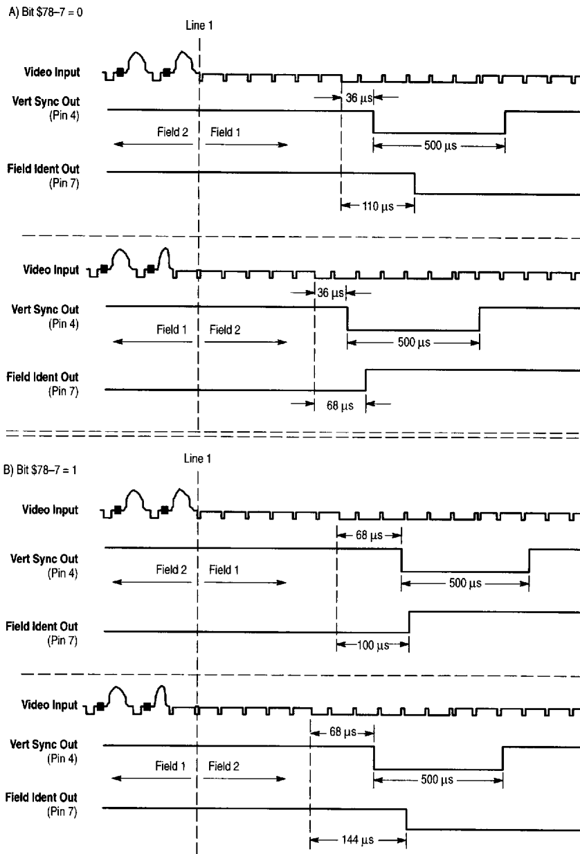
Figure 33. Vertical Timing (NTSC System)
