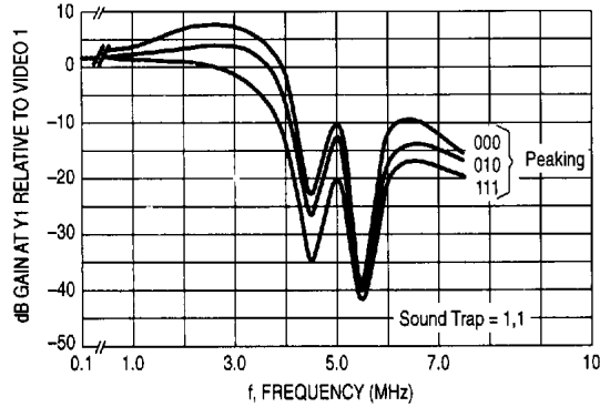
Figure 4. Composite Video Mode
