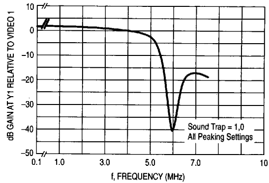
Figure 9. S-VHS Mode
