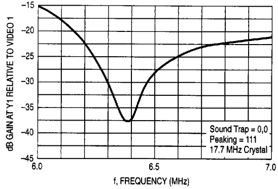
Figure 23. S-VHS Mode
