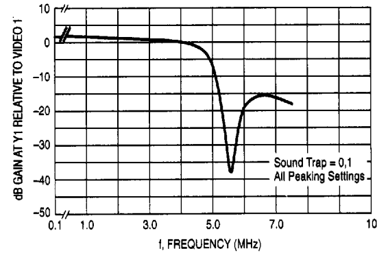
Figure 7. S-VHS Mode
