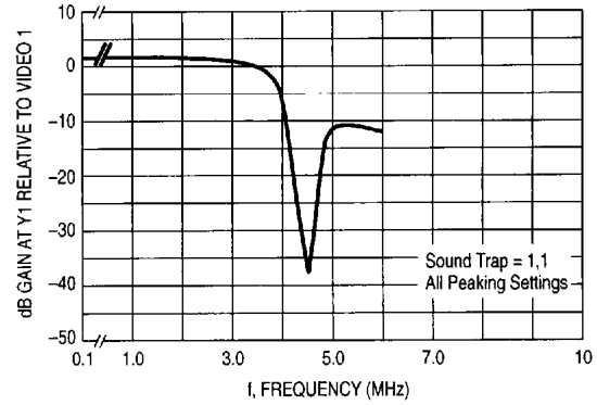
Figure 3. S-VHS Mode
