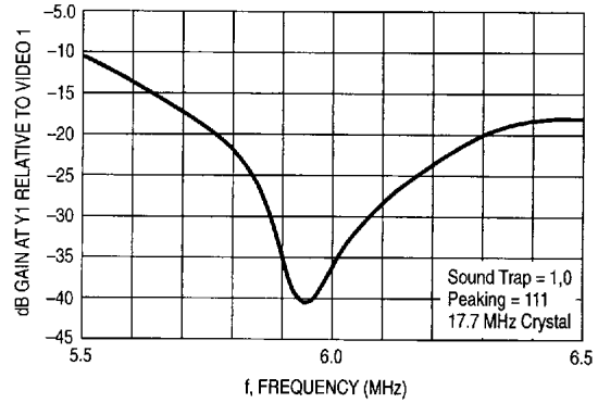
Figure 21. S-VHS Mode
