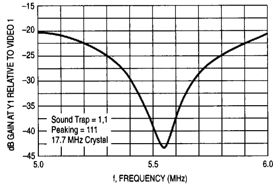
Figure 16. Composite Video Mode
