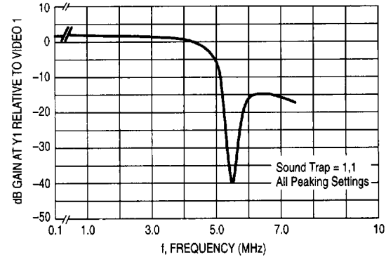
Figure 5. S-VHS Mode
