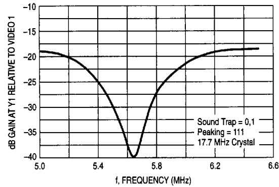
Figure 18. Composite Video Mode
