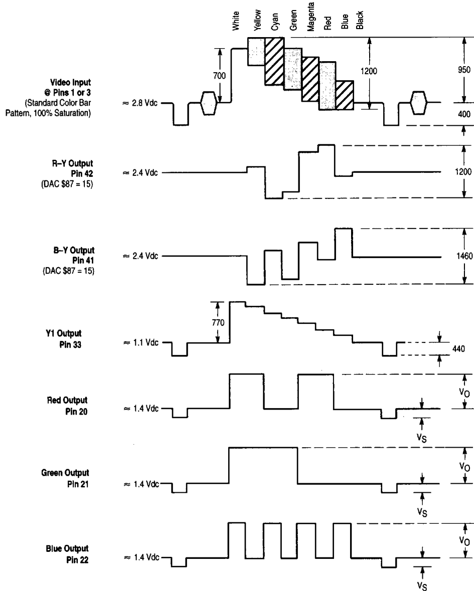
Figure 45. Typical Waveforms
