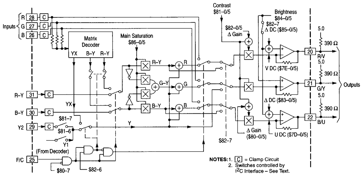
Figure 36. Color Difference Stage and Outputs
