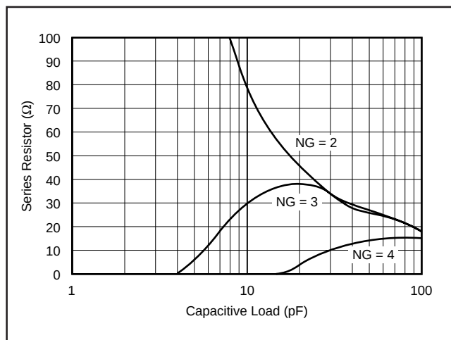
FIGURE 10. Required R_S vs Noise Gain
