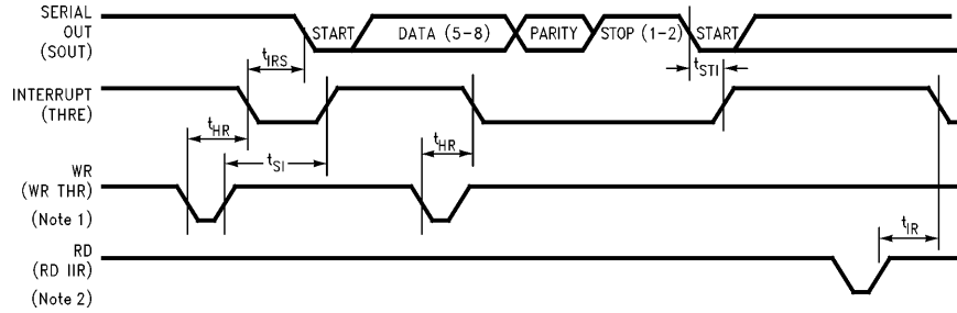
FIGURE 9-5. Transmitter Timing
