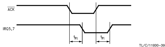
FIGURE 9-14. Compatible Mode Parallel Port Interrupt Timing
