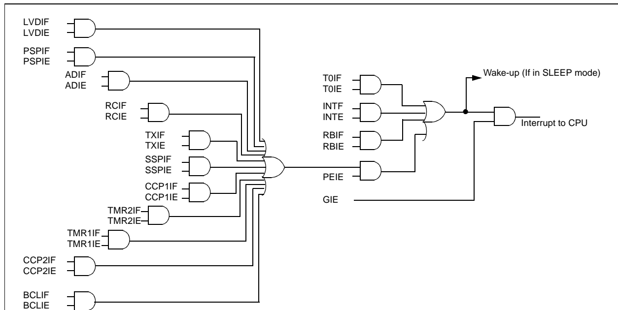
FIGURE 12-11: INTERRUPT LOGIC
