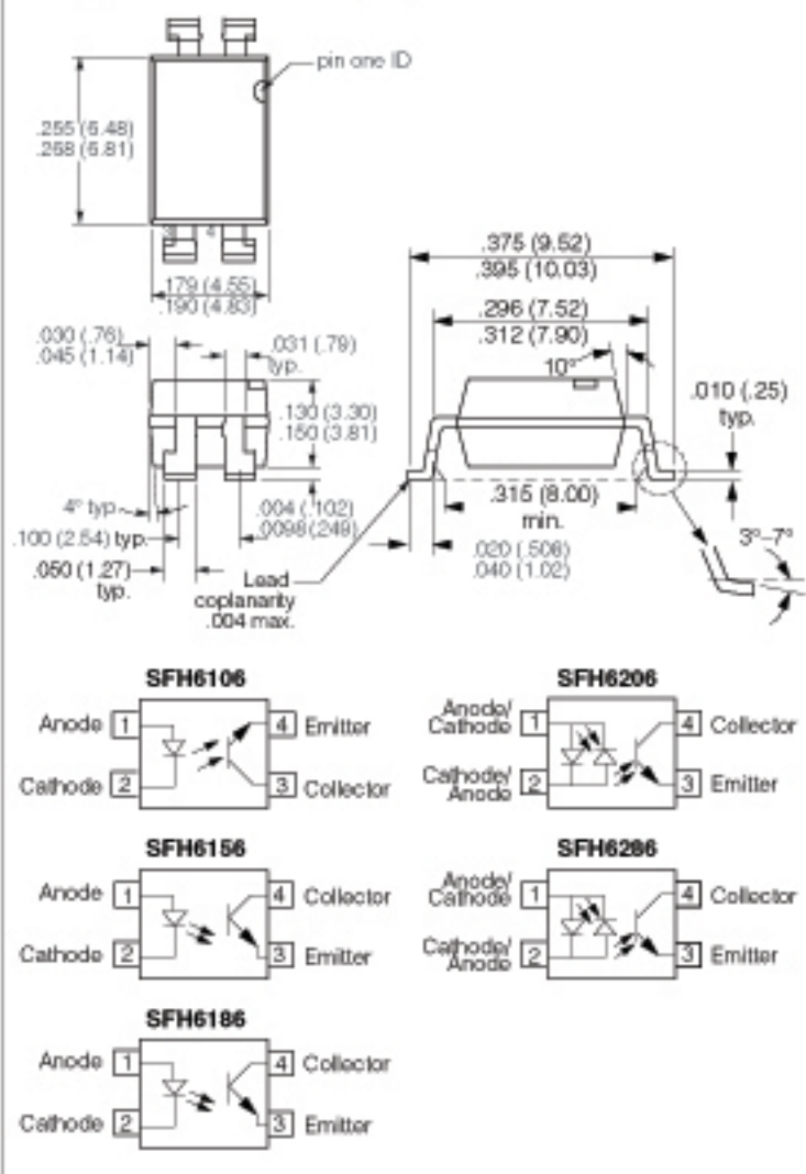
Package Dimensions in Inches (mm)
